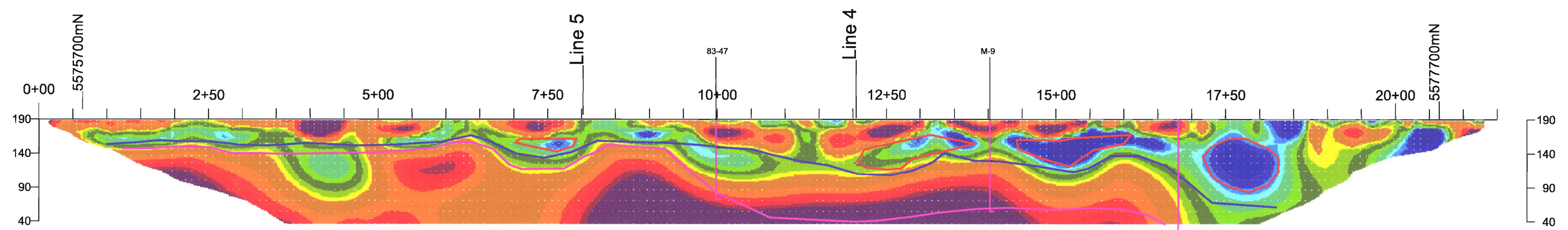
Interpreted Resistivity Profiles
