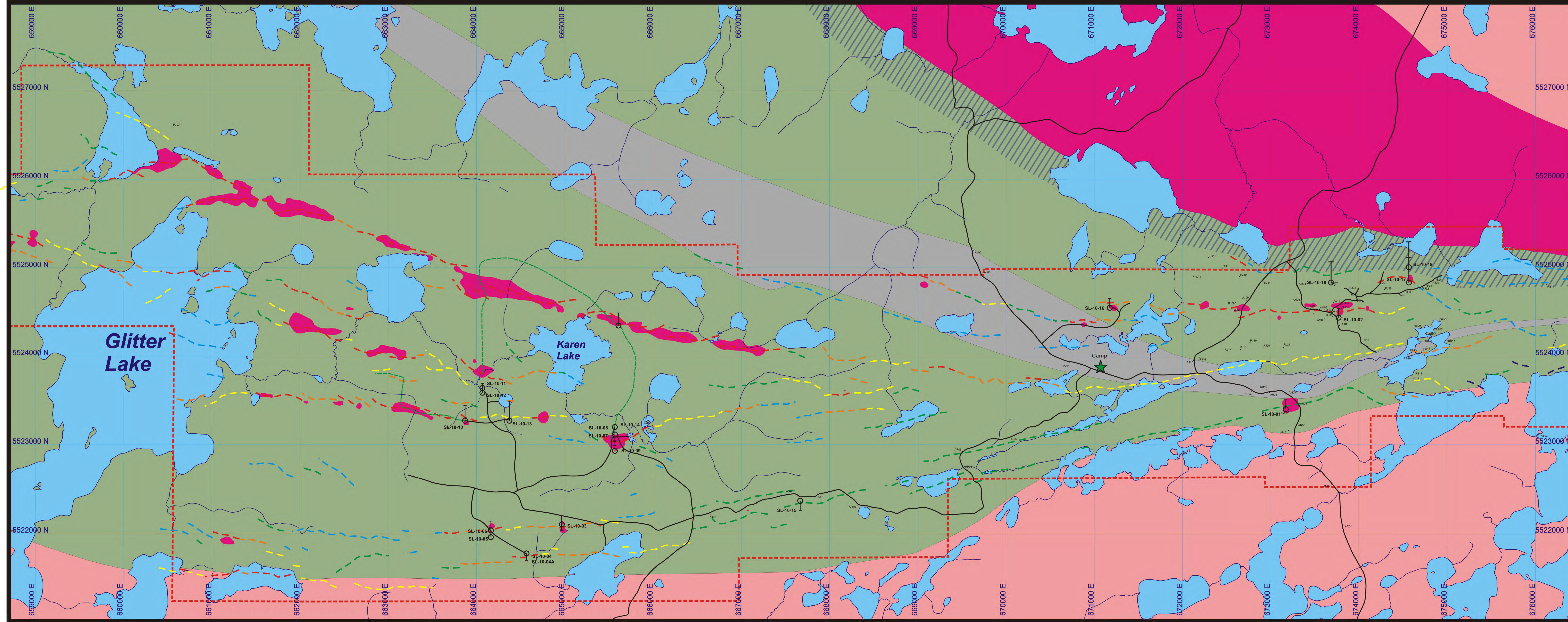
Figure 3: Sturgeon Lake Regional Geology
