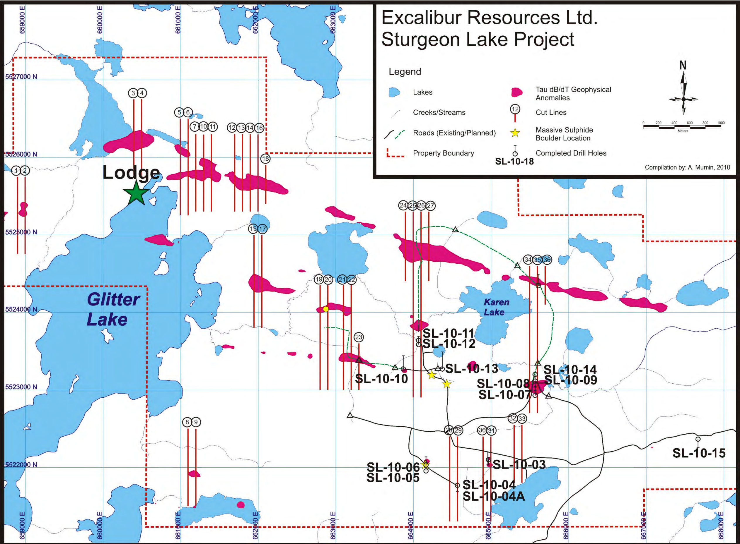
Figure 5: Sturgeon Lake 2010 drill hole locations.
