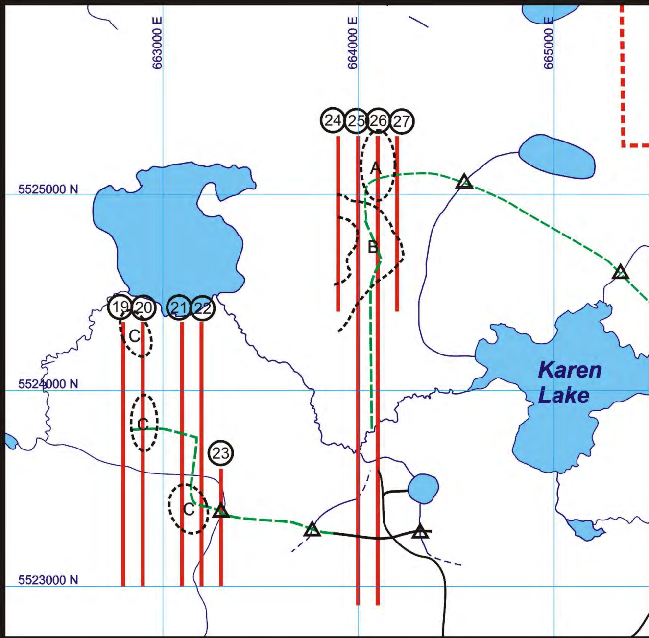
Figure 8: SGH apical anomalies for lines 19 to 27. Anomalies “A” and “B” have a SGH rating of 2.0, and anomalies “C” have a rating of 6.0, which is the highest possible rating, and represents excellent targets for follow-up drilling.
