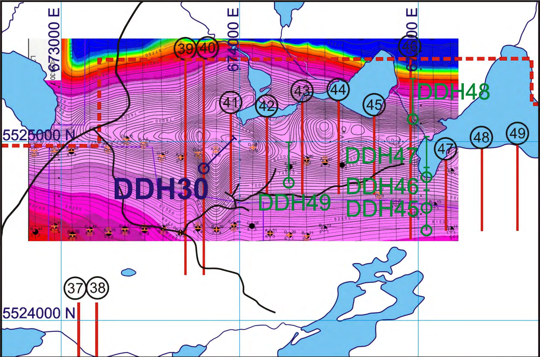
Figure 12: Drill setup at DDH30 with the Total Magnetic Intensity map from the 2009 geophysical survey. DDH30 is setup to drill across the intersection of the strong N-S magnetic liniment visible between lines 40 and 41, and the E-W trending iron formation.
