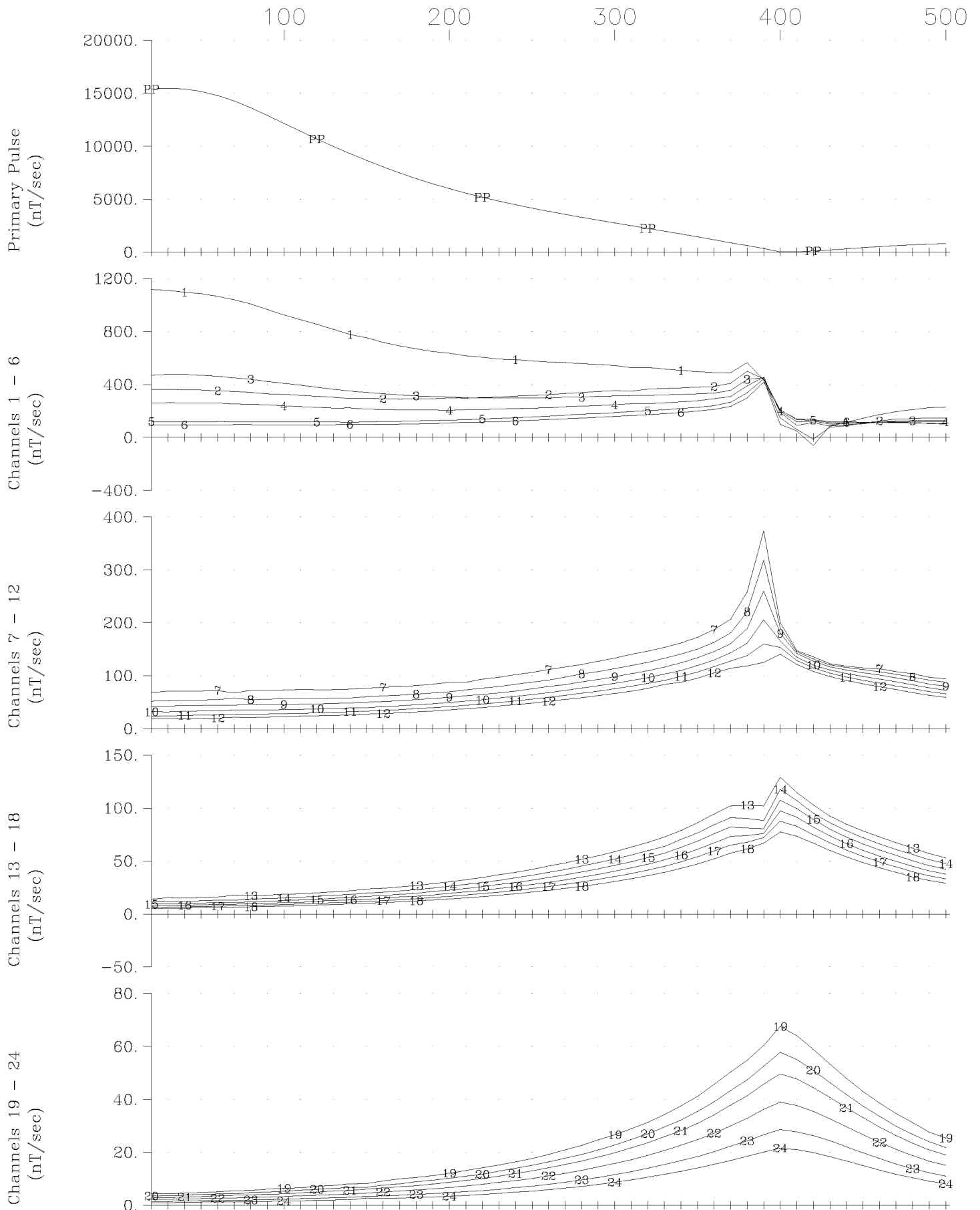
Ursa Major Minerals Inc. Shakespeare East Property Loop 2, Hole U-03-121 Z Component Crone Geophysics & Exploration Ltd.
