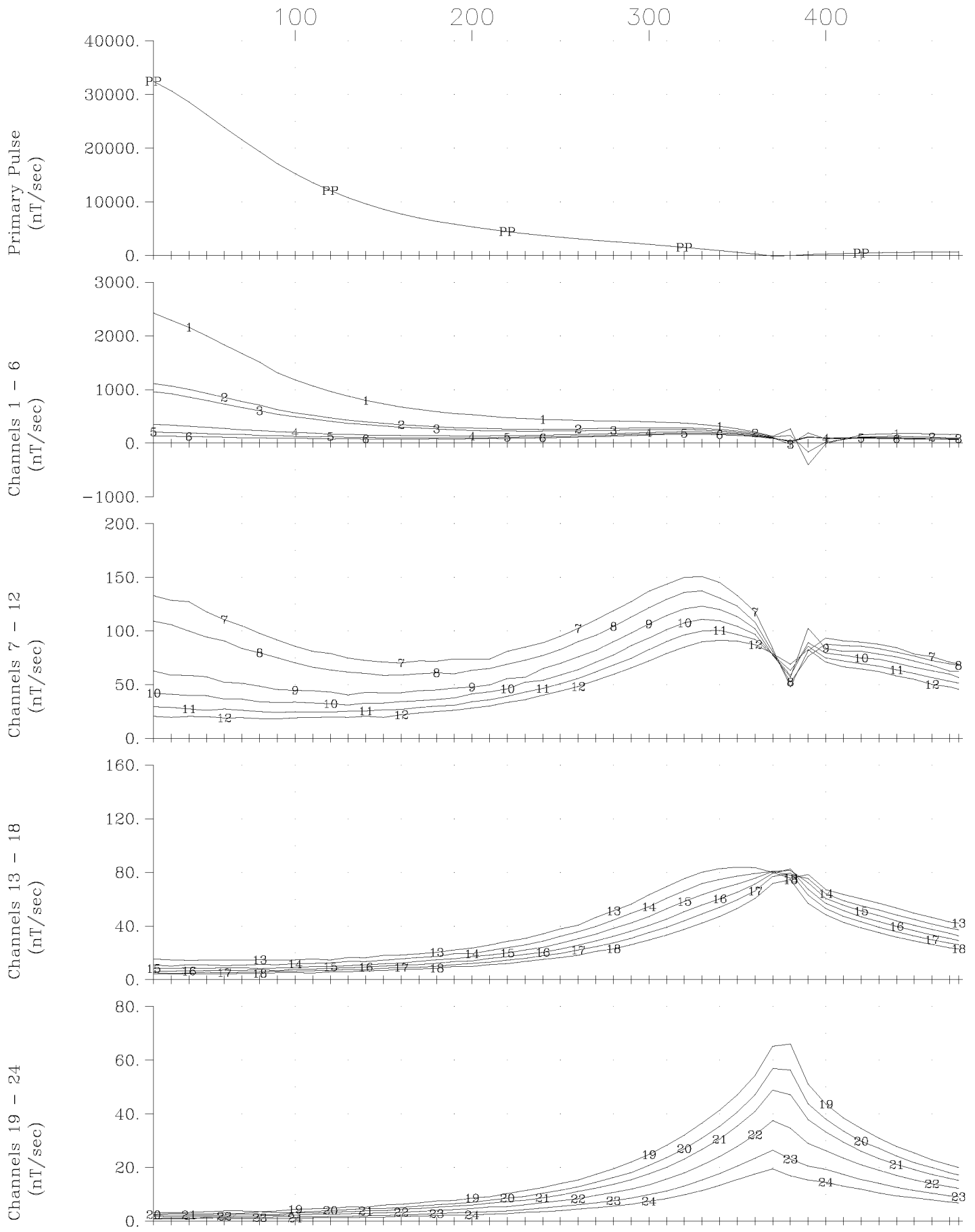
Ursa Major Minerals Inc. Shakespeare East Property Loop 1, Hole U-03-120 Z Component Crone Geophysics & Exploration Ltd.
