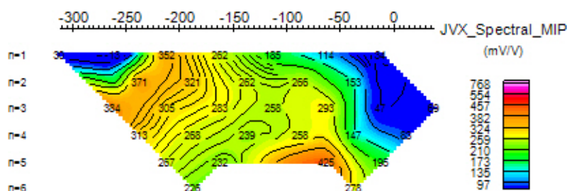
JVX_Spectral_MIP (mV/V)
