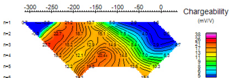
Chargeability (mV/V)
