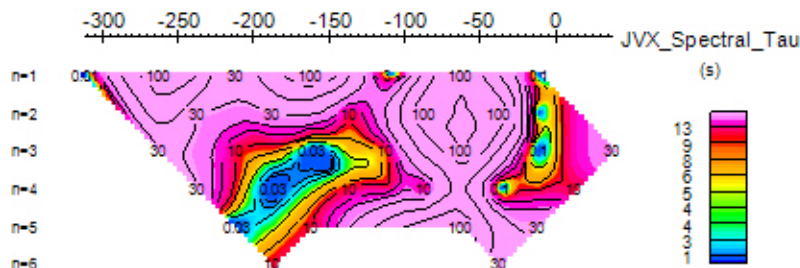
JVX_Spectral_Tau (s)
