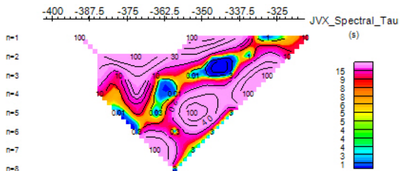
JVX_Spectral_Tau (s)
