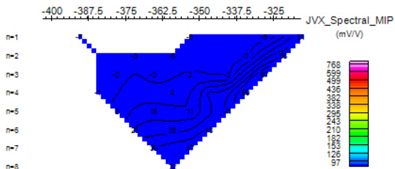
JVX_Spectral_MIP (mV/V)
