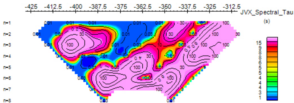
JVX_Spectral_Tau (s)
