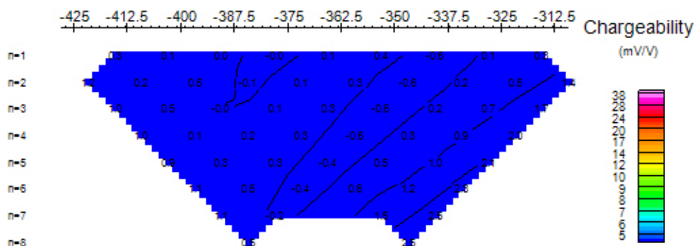
Chargeability (mV/V)
