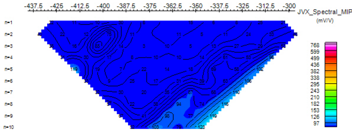
JVX_Spectral_MIP (mV/V)
