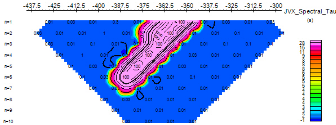
JVX_Spectral_Tau (s)
