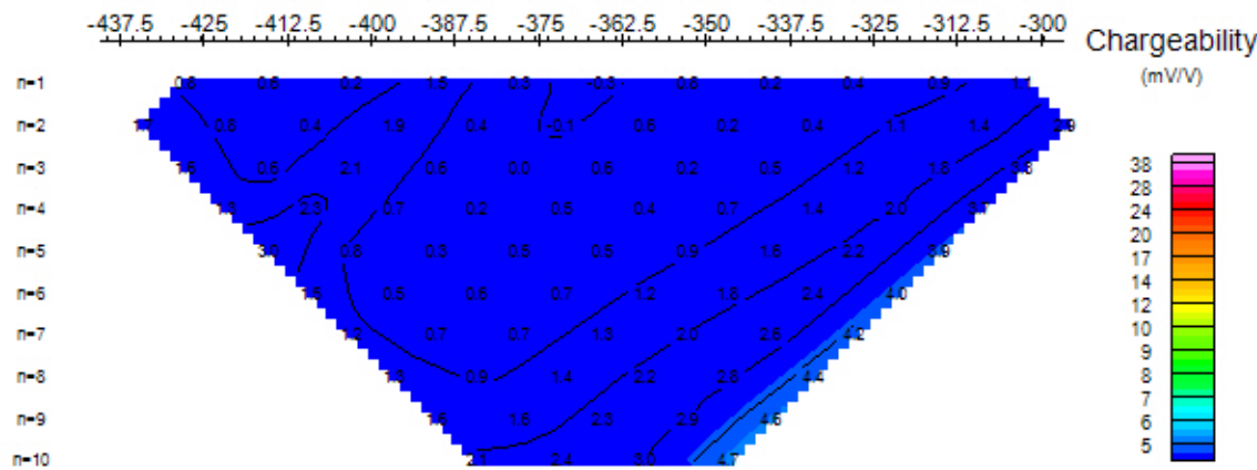
Chargeability (mV/V)
