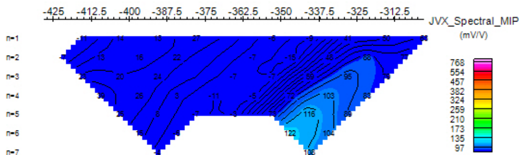
JVX_Spectral_MIP (mV/V)
