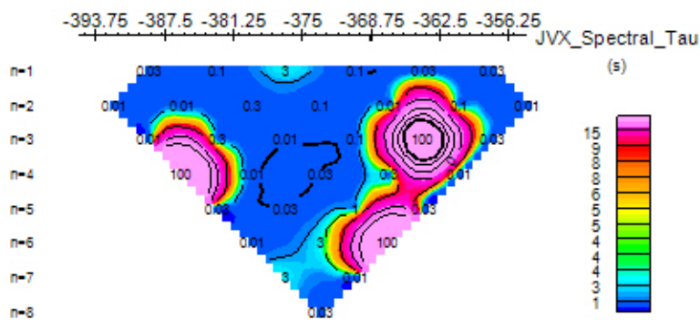
JVX_Spectral_Tau (s)
