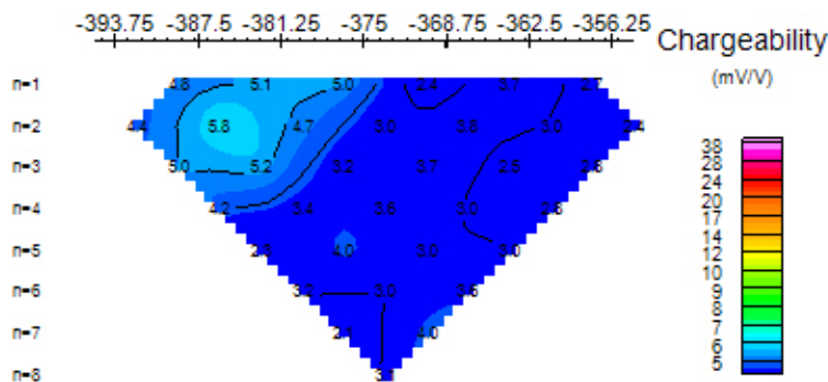
Chargeability (mV/V)
