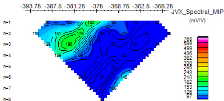
JVX_Spectral_MIP (mV/V)
