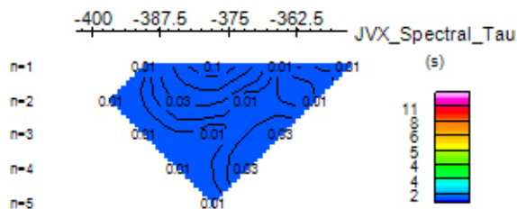
JVX_Spectral_Tau (s)
