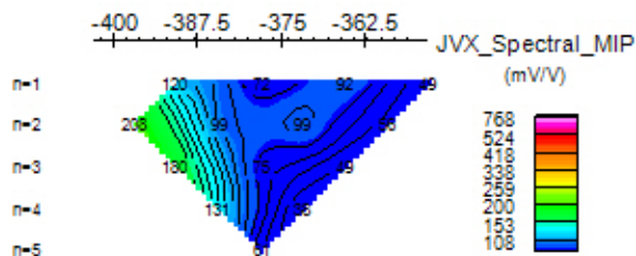
JVX_Spectral_MIP (mV/V)
