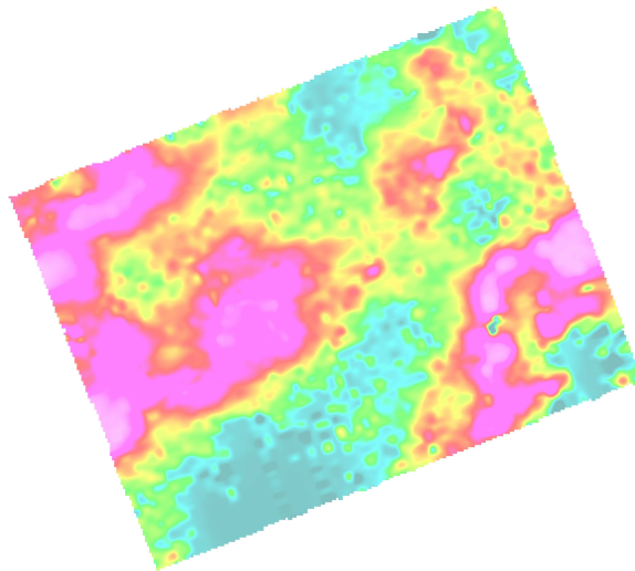
Figure 2. Apparent Conductivity derived from dB/dt Z-Coil Channel 01
