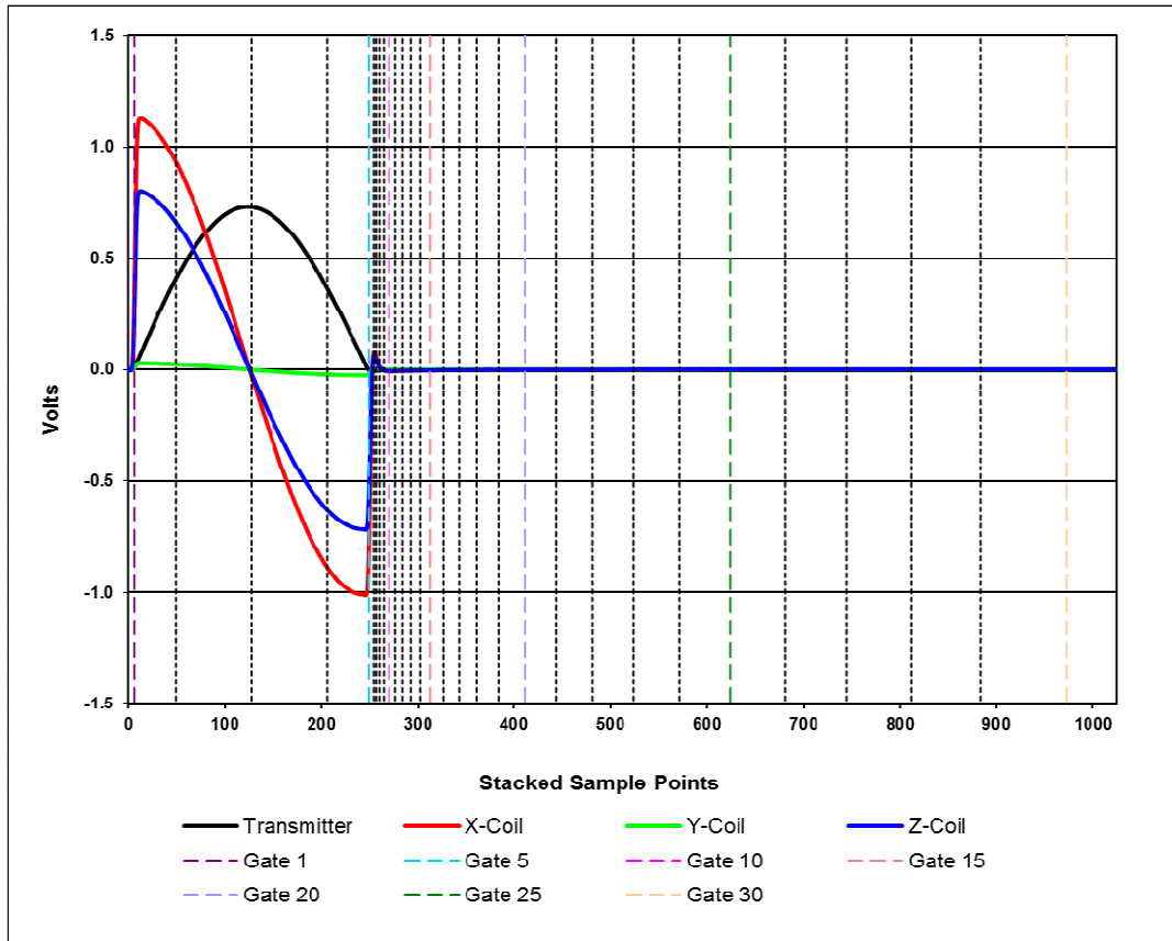
Figure 5: GEOTEM® Waveform and response with gate centres showing positions in sample points.
