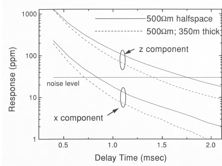
Fig. 2. The response for a 500 \Omega\cdot\text{m} half-space (solid line) and a 500 \Omega\cdot\text{m} layer of thickness 350 m overlying a resistive half-space (dashed line). The z-component responses are the two curves with the larger amplitudes and the two x-component response curves are 6 to 10 times smaller than the corresponding z component. A noise level of 30 ppm is considered to be typical of both components in the absence of strong spherics.
