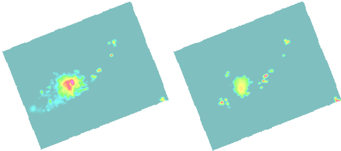
Figure 1. Decay Constant ( \tau ) derived from dB/dt Z-Coil Channels 8-30 (left) and B-Field Z-Coil Channels 16-30 (right)
