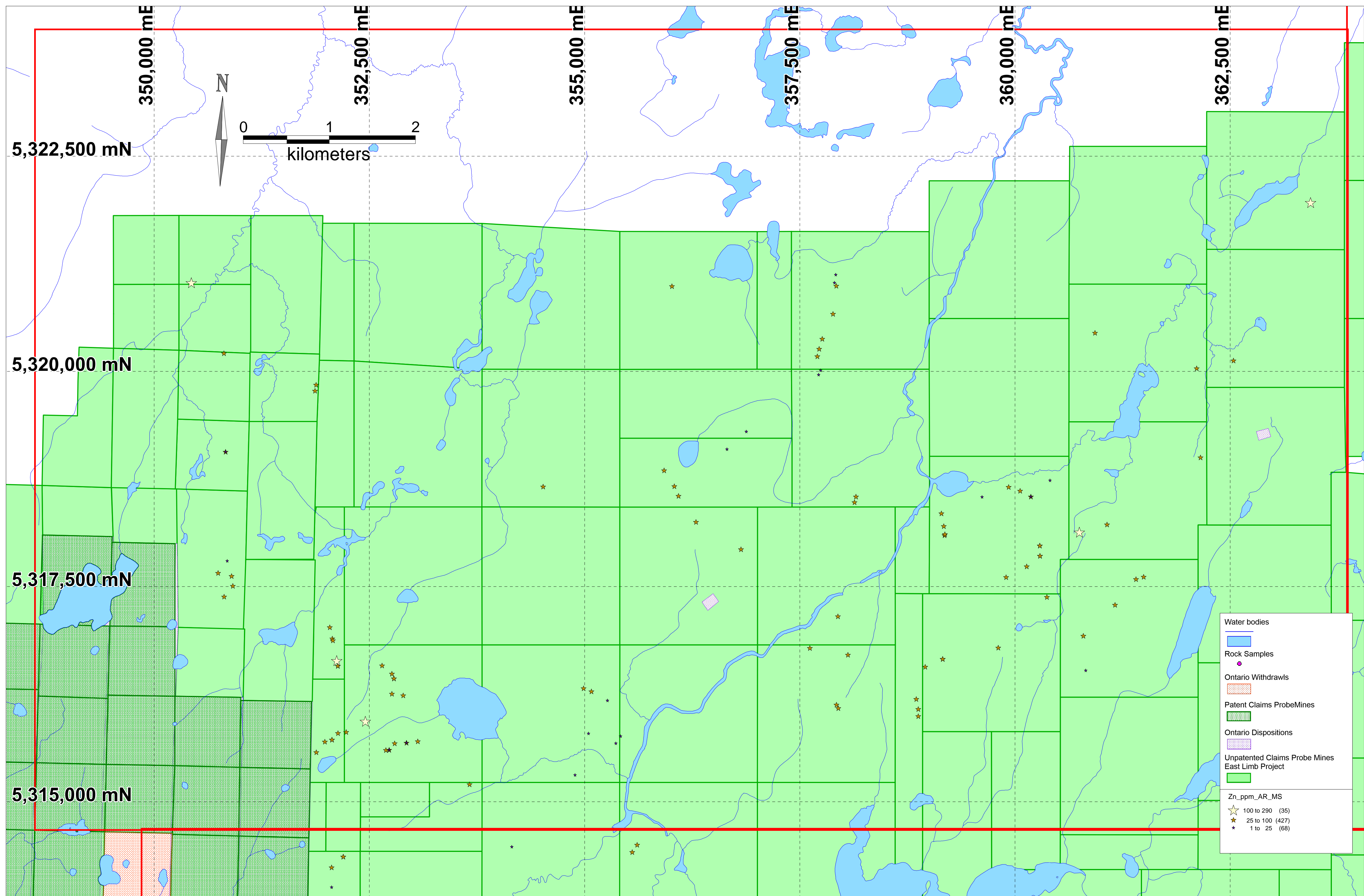
Appendix 3 - Rock Samples Zn ppm by Aqua RegiaMS
