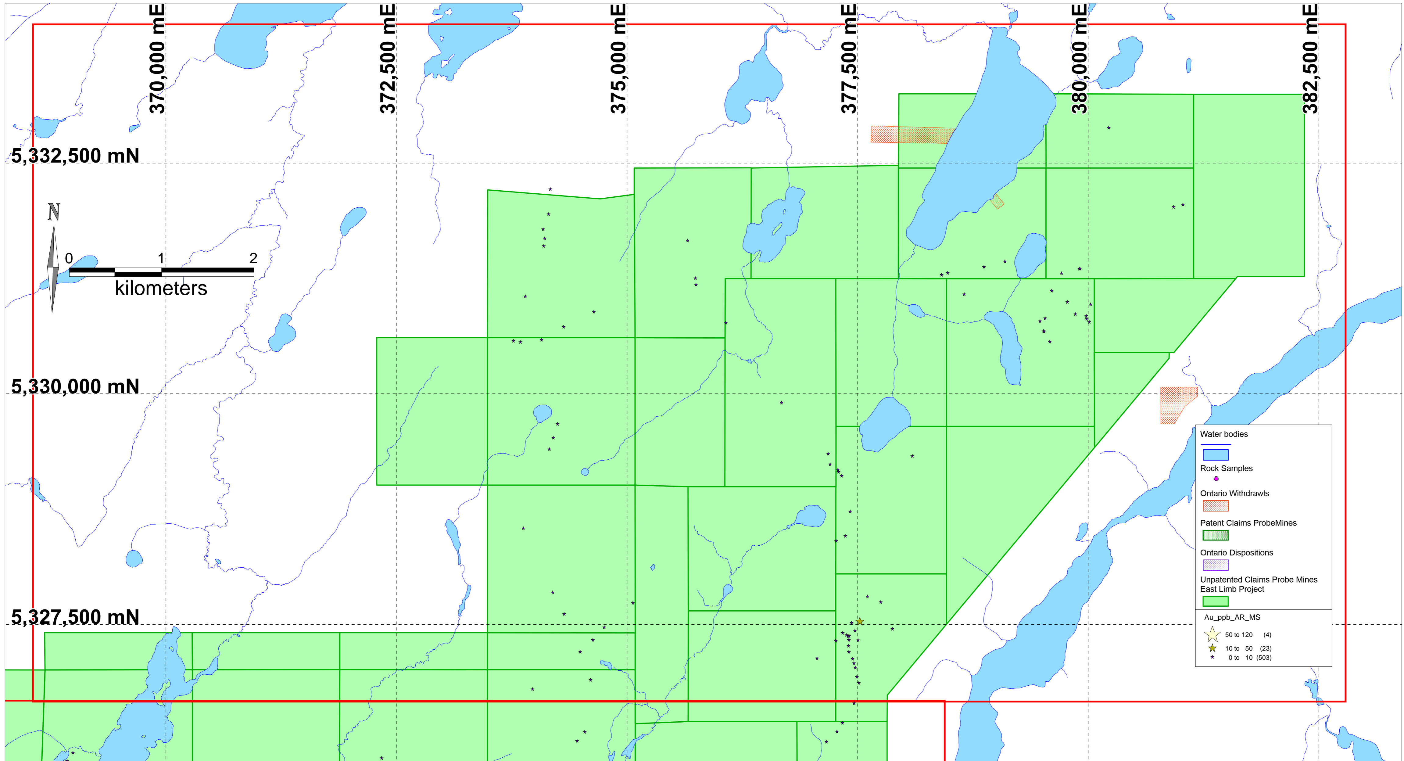
Appendix 3 - Rock Samples Au ppb by Aqua RegiaMS
