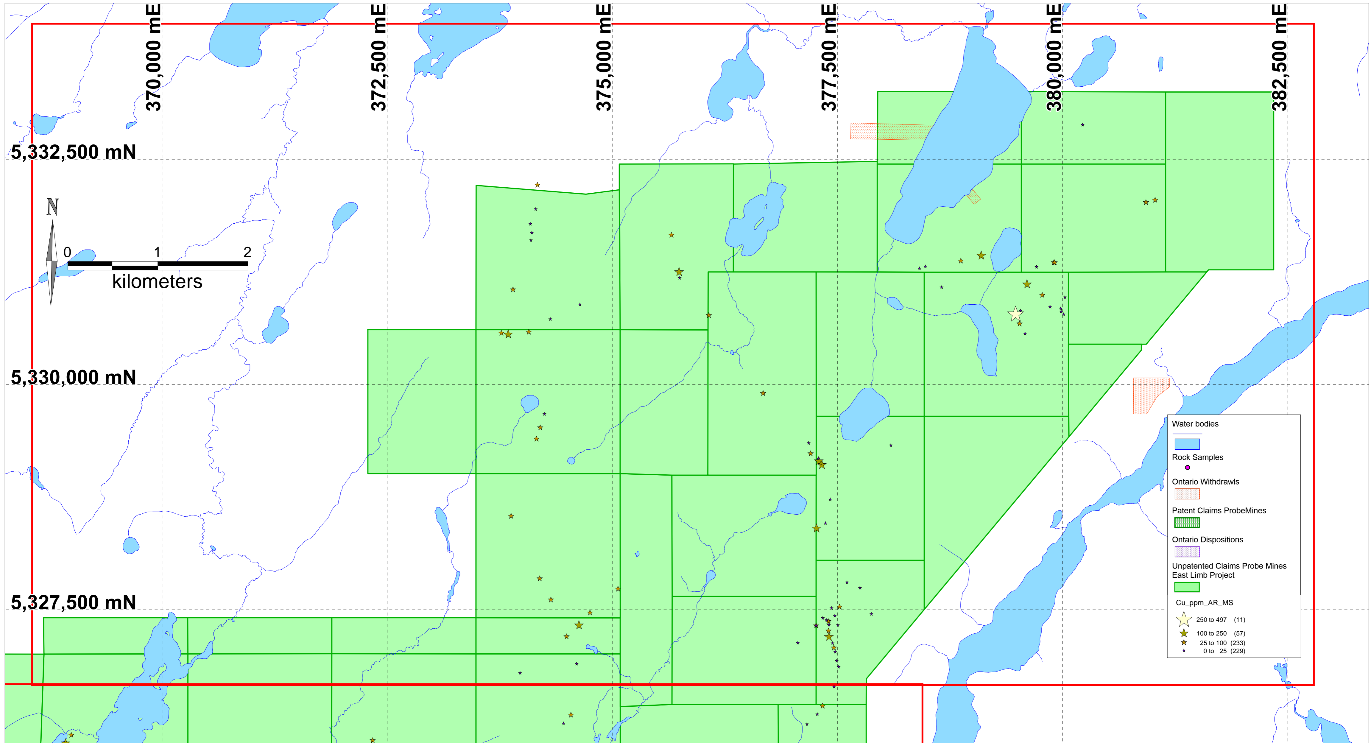
Appendix 3 - Rock Samples Cu ppm by Aqua RegiaMS
