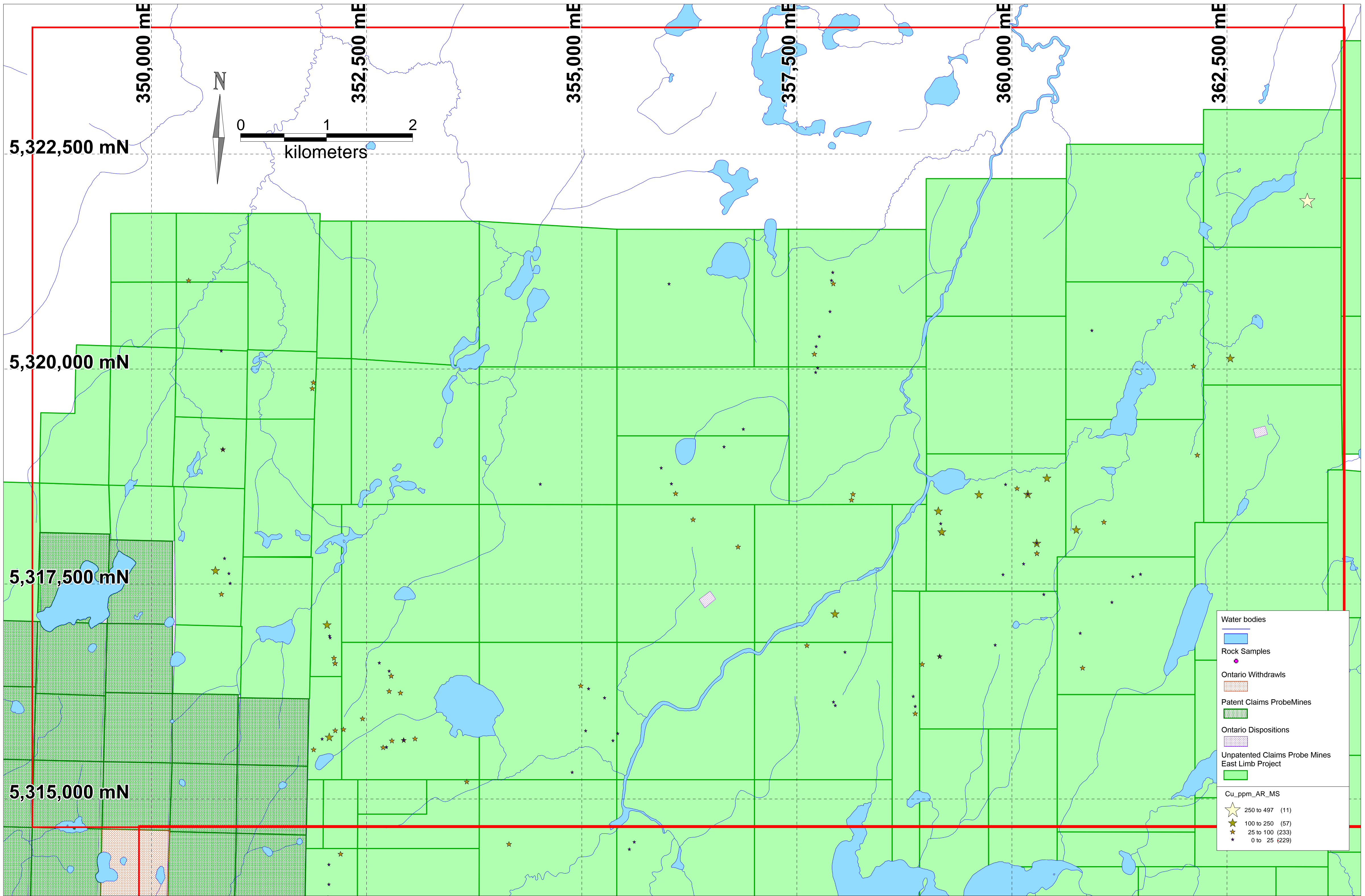
Appendix 3 - Rock Samples Cu ppm by Aqua RegiaMS
