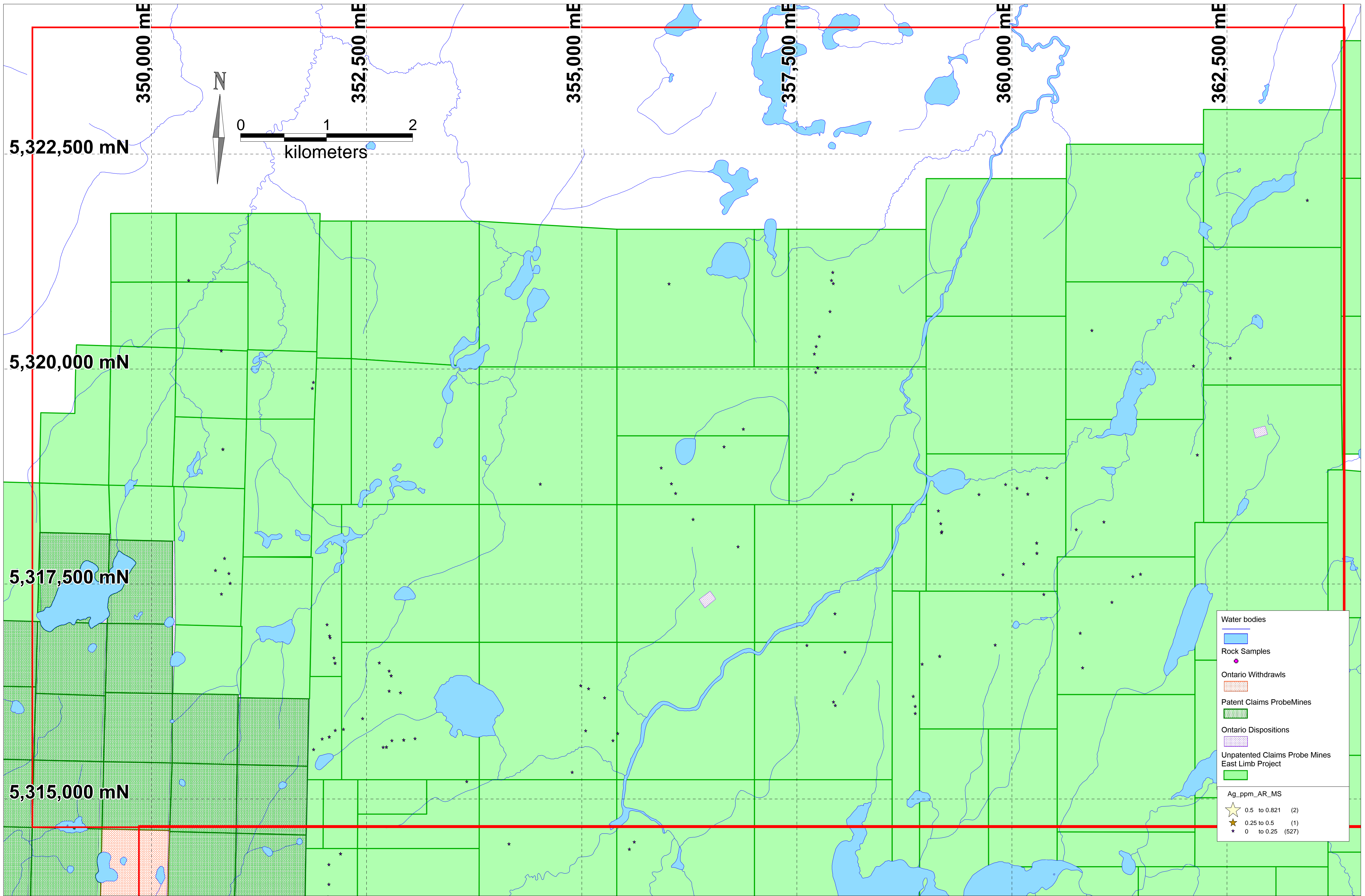
Appendix 3 - Rock Samples Au ppb by Aqua RegiaMS
