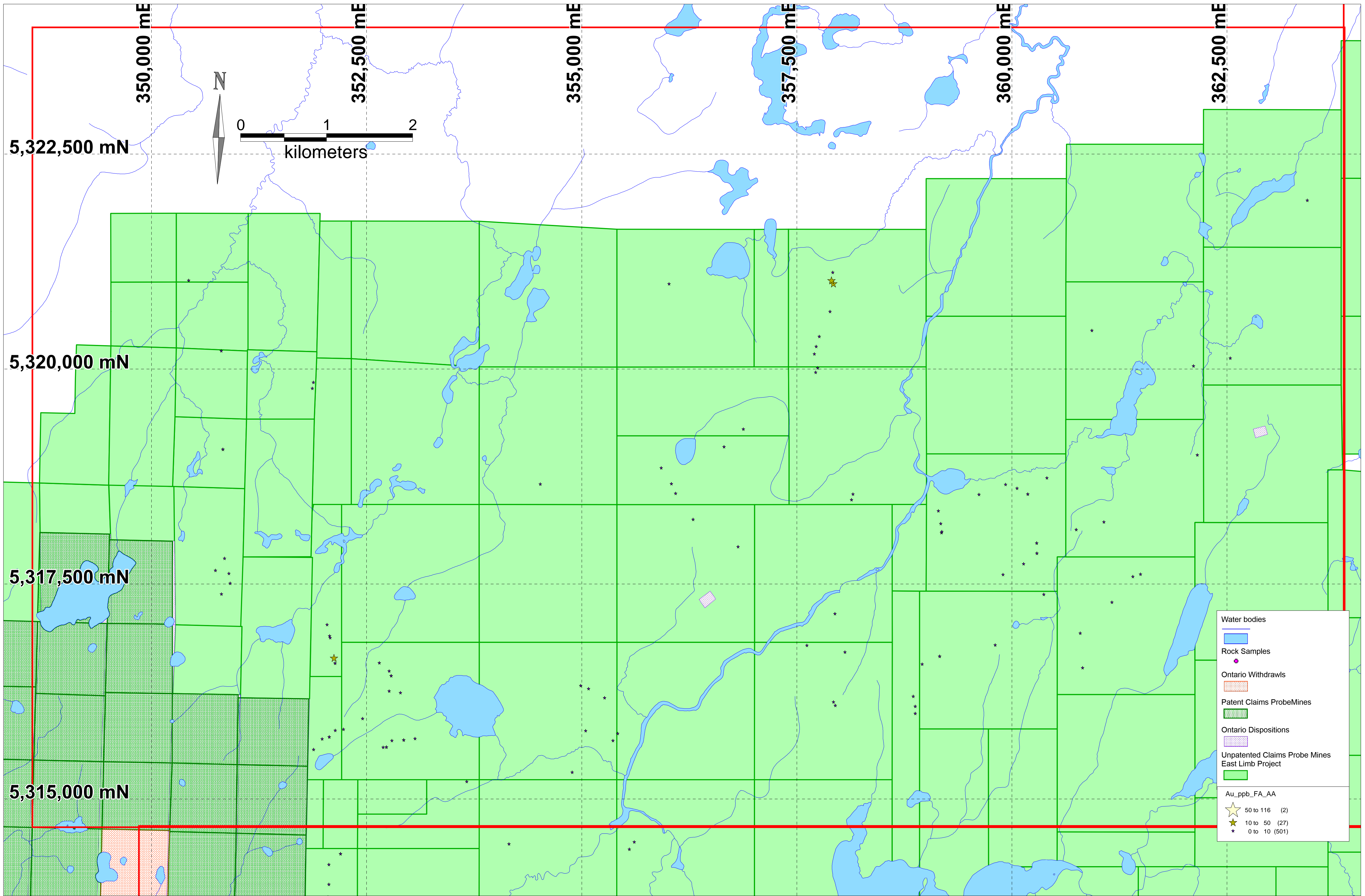
Appendix 3 - Rock Samples Au ppb by FA-AA
