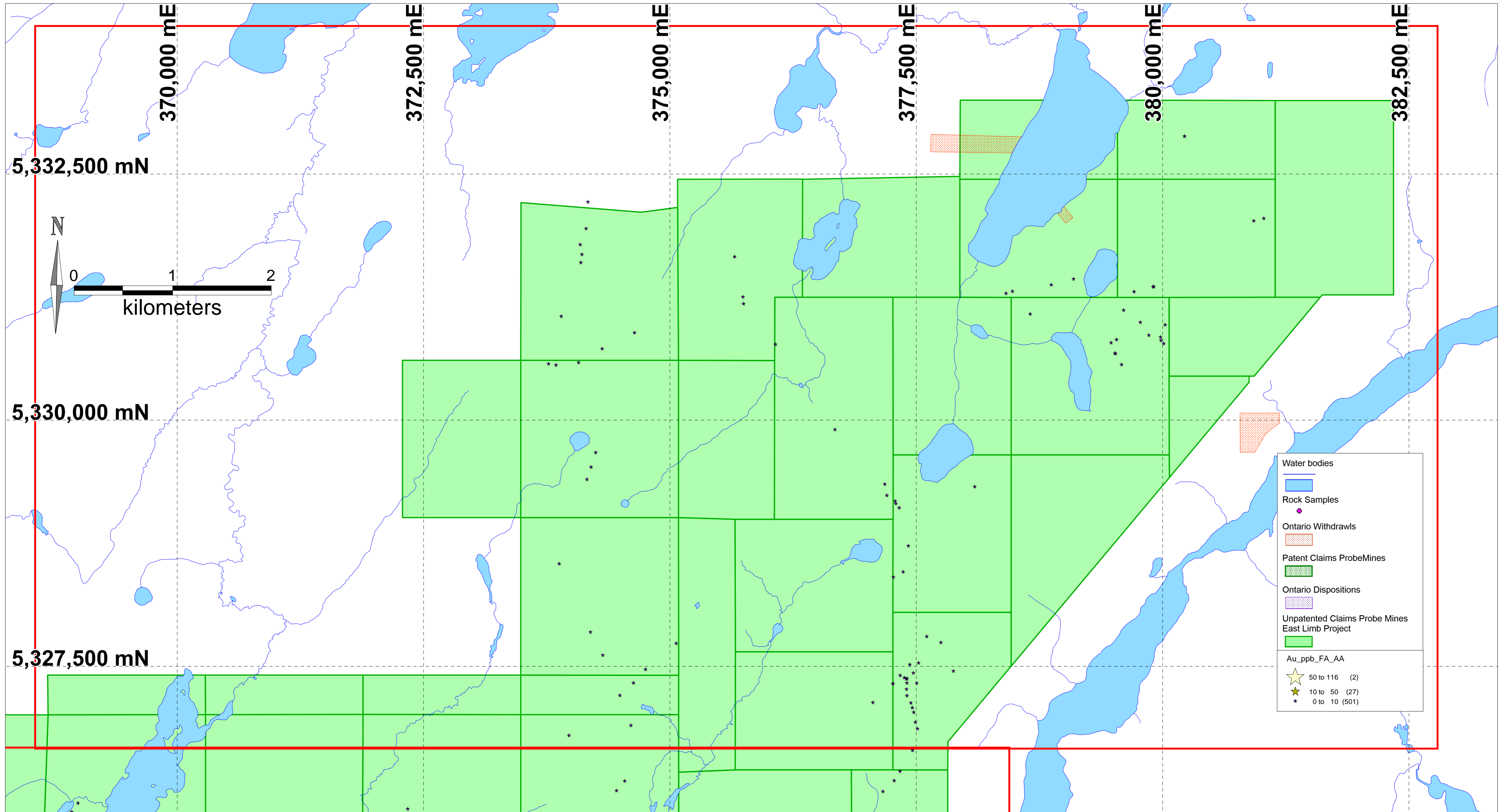
Appendix 3 - Rock Samples Au ppb by FA-AA
