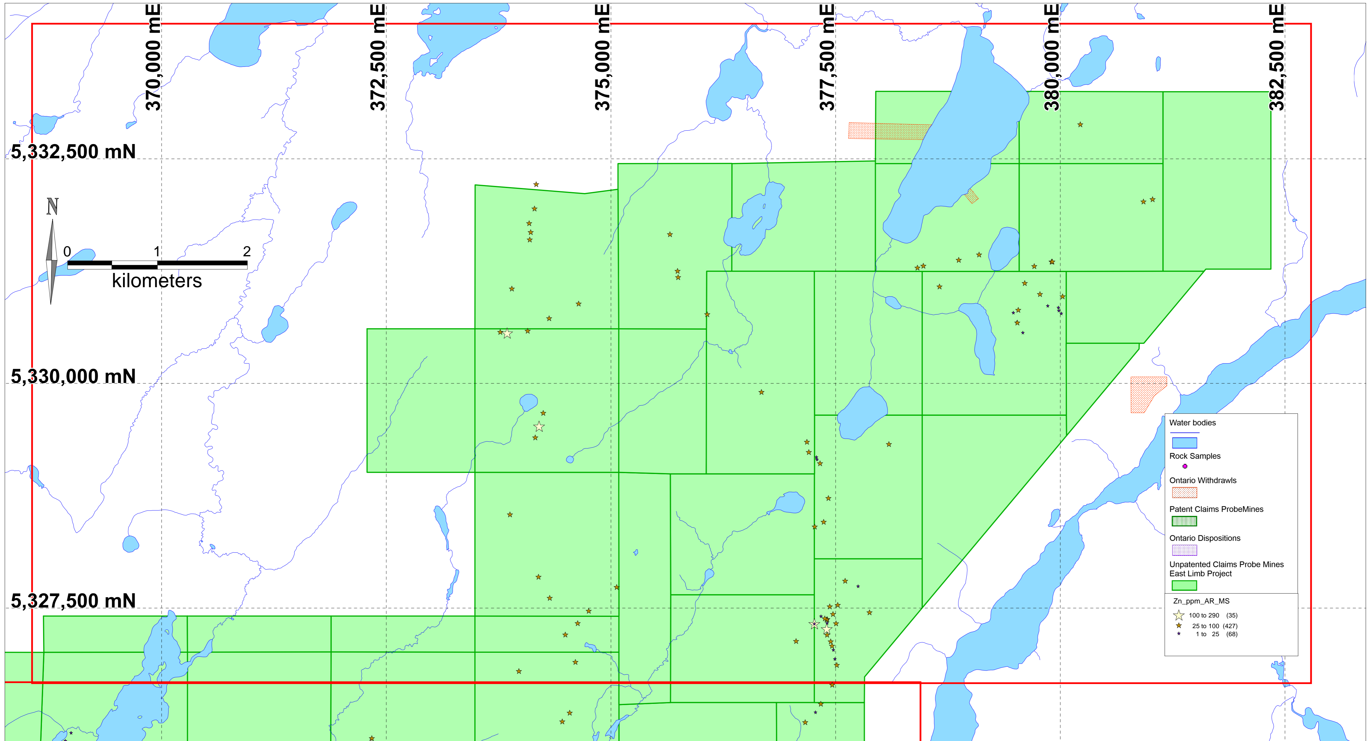
Appendix 3 - Rock Samples Zn ppm by Aqua RegiaMS
