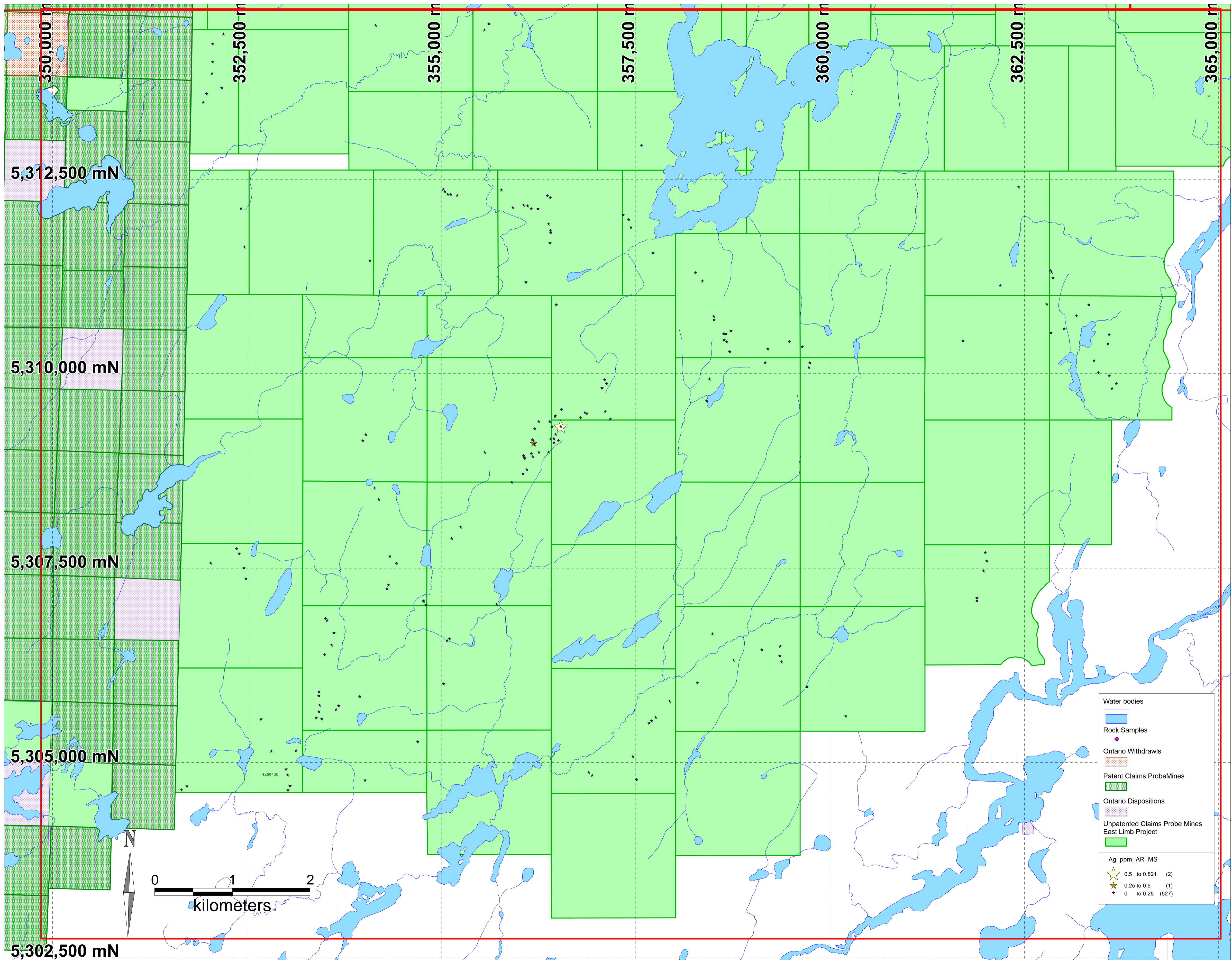
Appendix 3 - Rock Samples Ag ppm by Aqua RegiaMS
