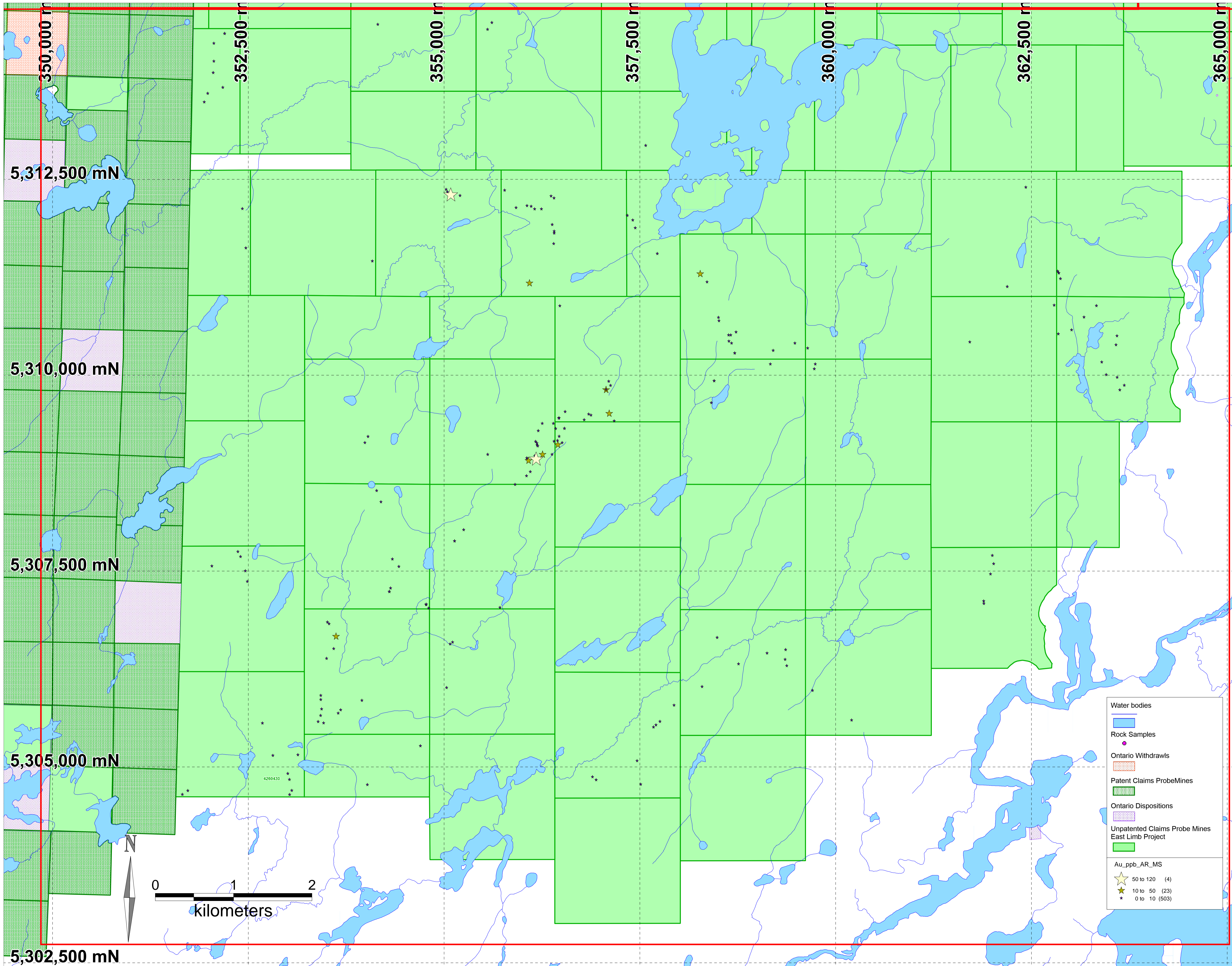
Appendix 3 - Rock Samples Au ppb by Aqua RegiaMS
