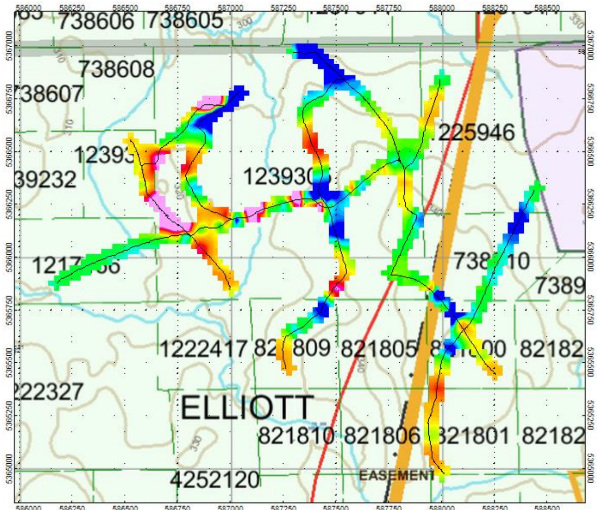
Figure 2: VLF EM In-Phase Readings
