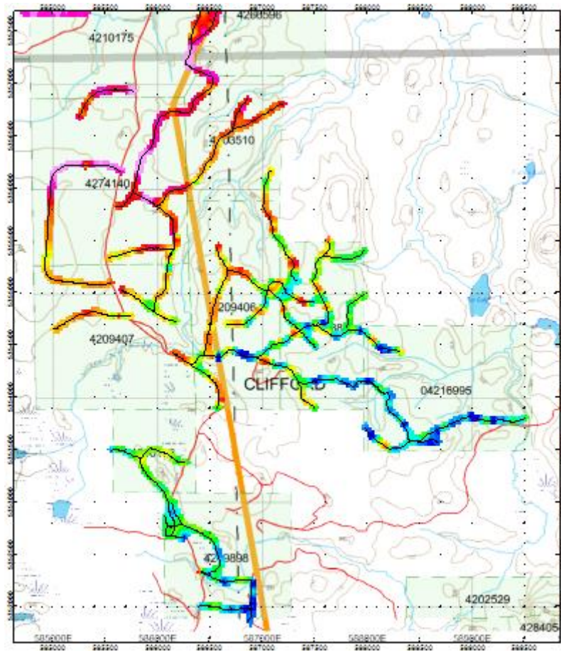
Figure 2: Magnetometer Readings
