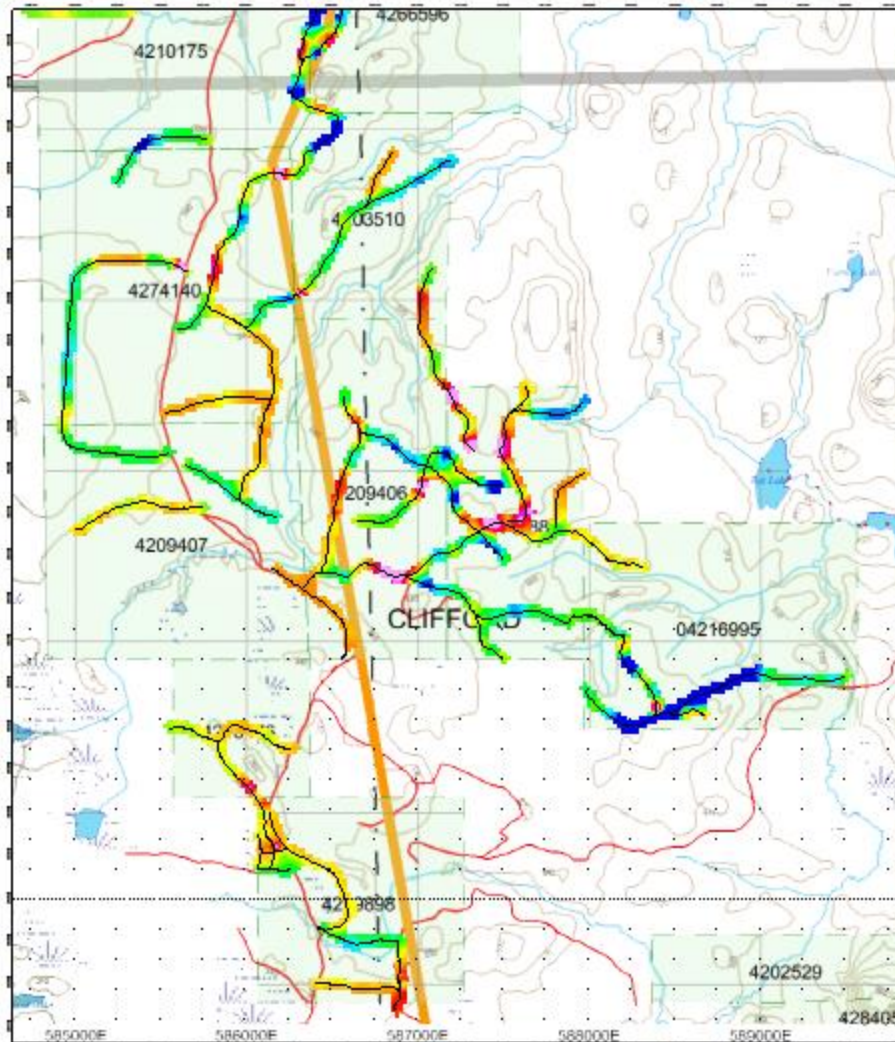
Figure 2: VLF EM In-Phase Readings
