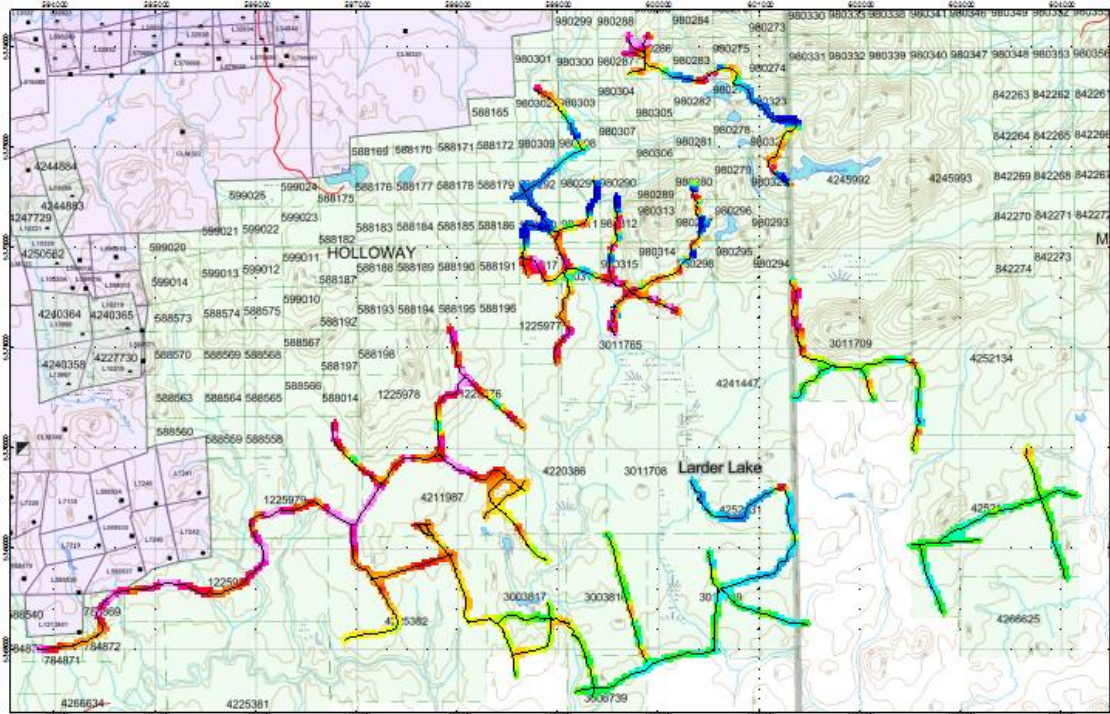
Figure 2: Magnetometer Readings
