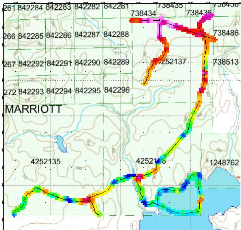
Figure 2: Magnetometer Readings
