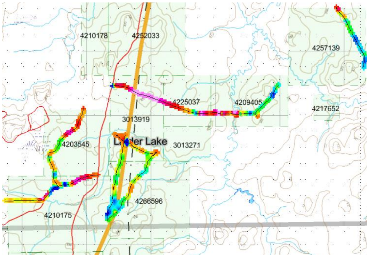
Figure 2: Magnetometer Readings
