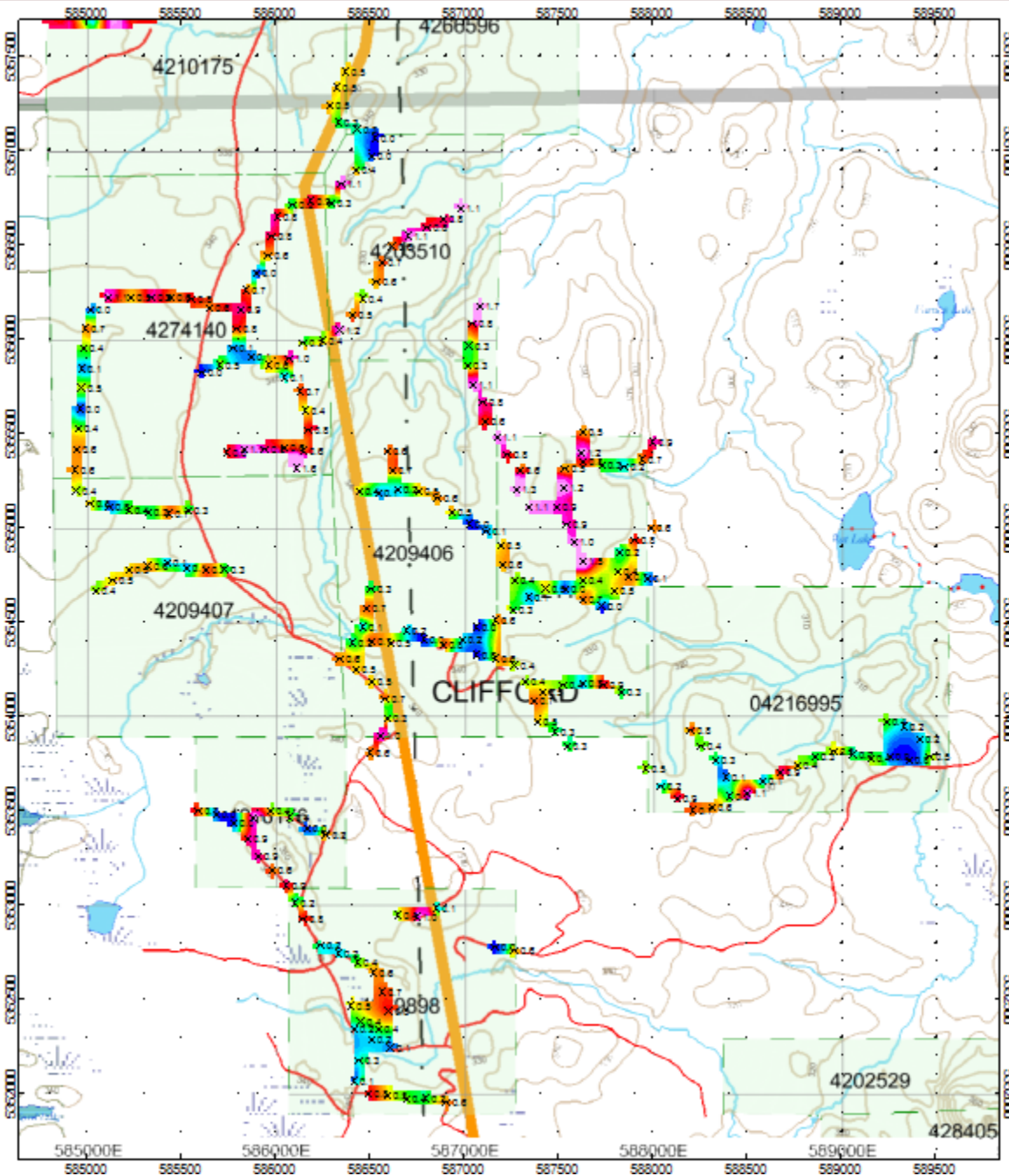
Figure 3: Spectrometer Uranium Readings
