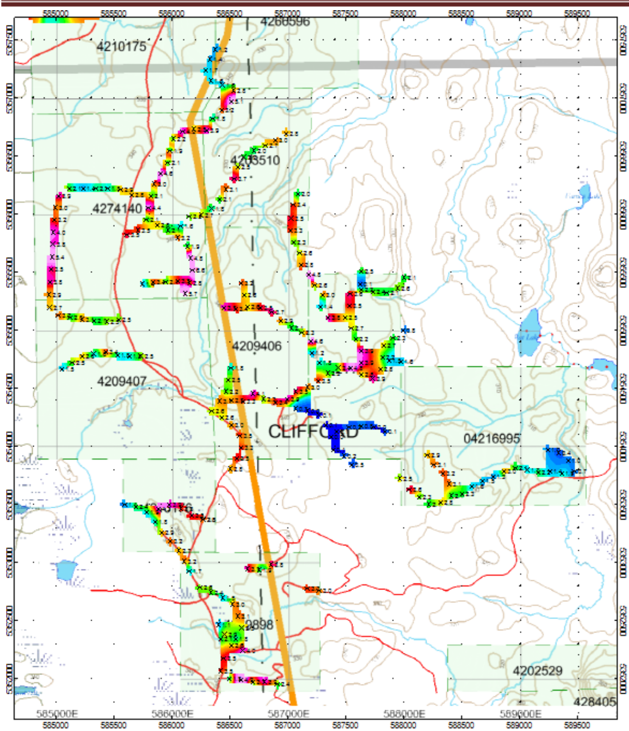
Figure 4: Spectrometer Thorium Readings
