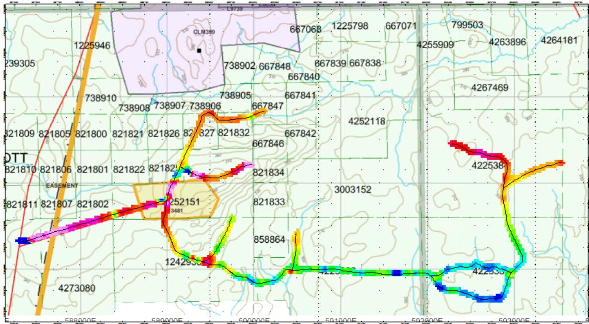
Figure 2: Magnetometer Readings
