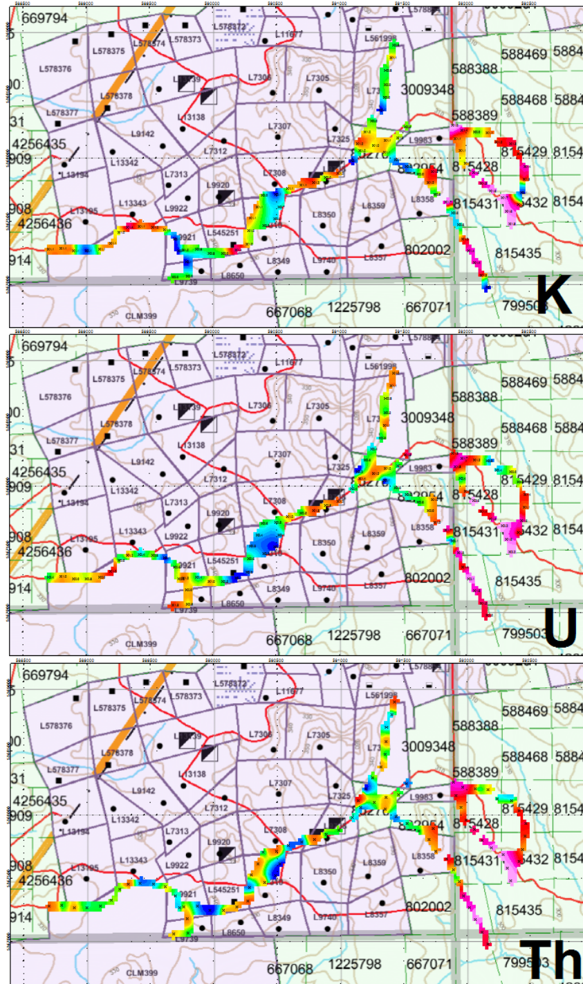
Figure 2: Spectrometer Readings
