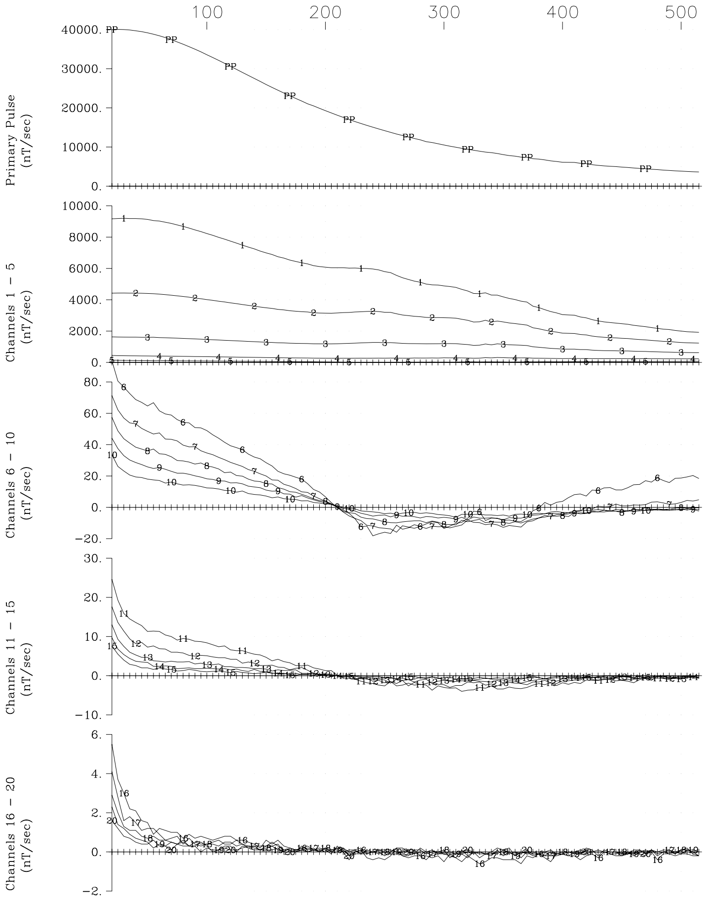
Transition Metals Sunday Lake Loop 2014-North, Hole SL-13-002 Z Component Crone Geophysics & Exploration Ltd.
