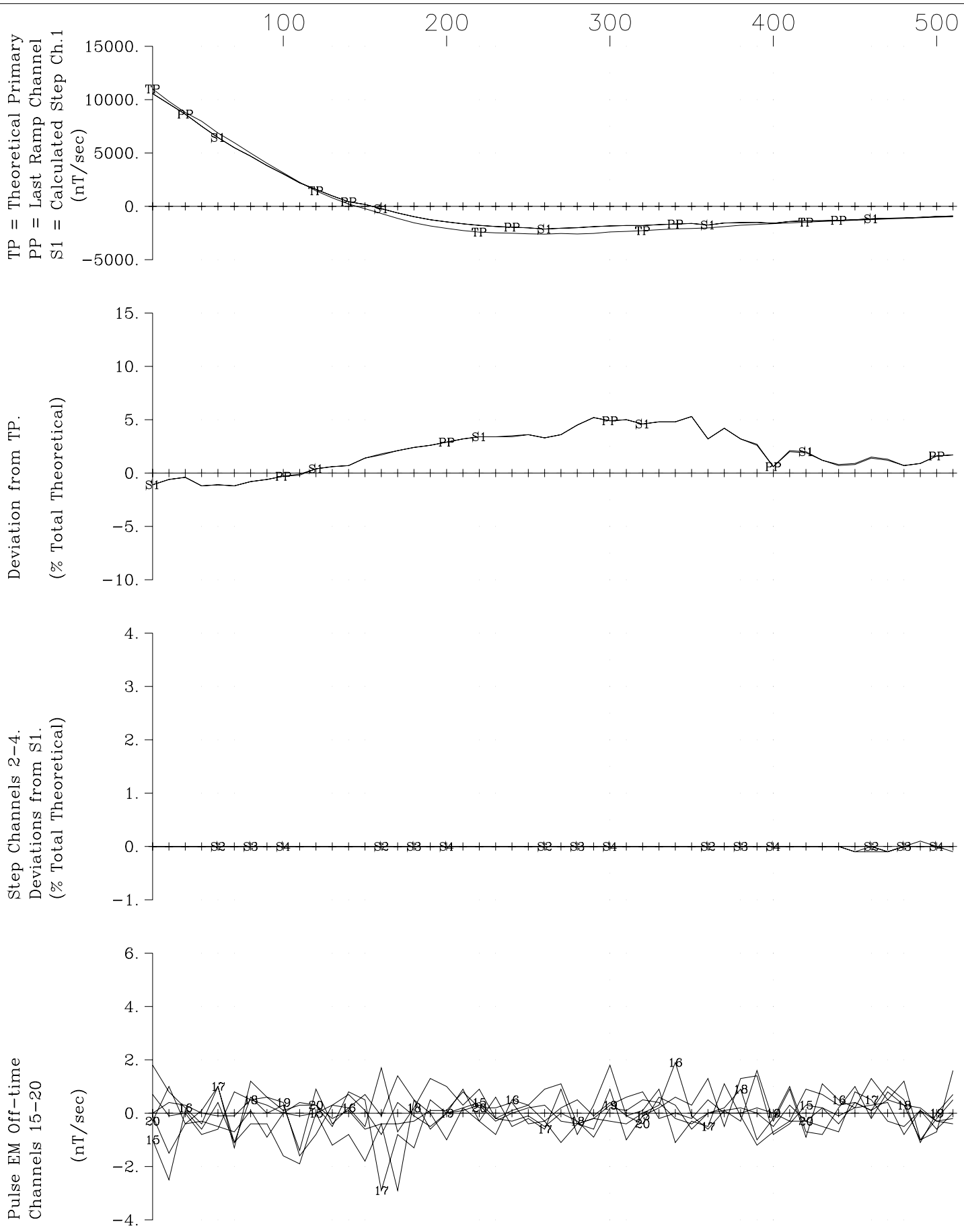
Transition Metals Sunday Lake Loop 2014-North, Hole SL-13-002 X Component Crone Geophysics & Exploration Ltd.
