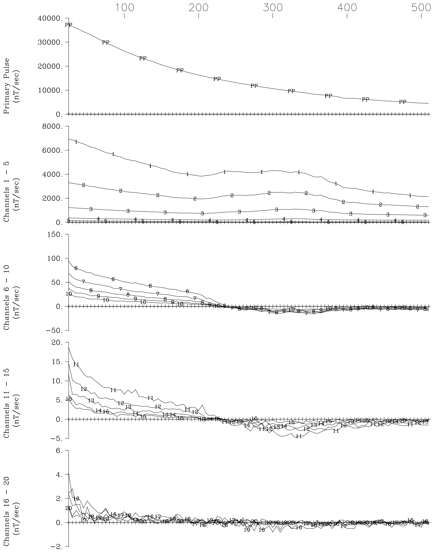
Transition Metals Sunday Lake Loop 2014-East, Hole SL-13-002 Z Component Crone Geophysics & Exploration Ltd.
