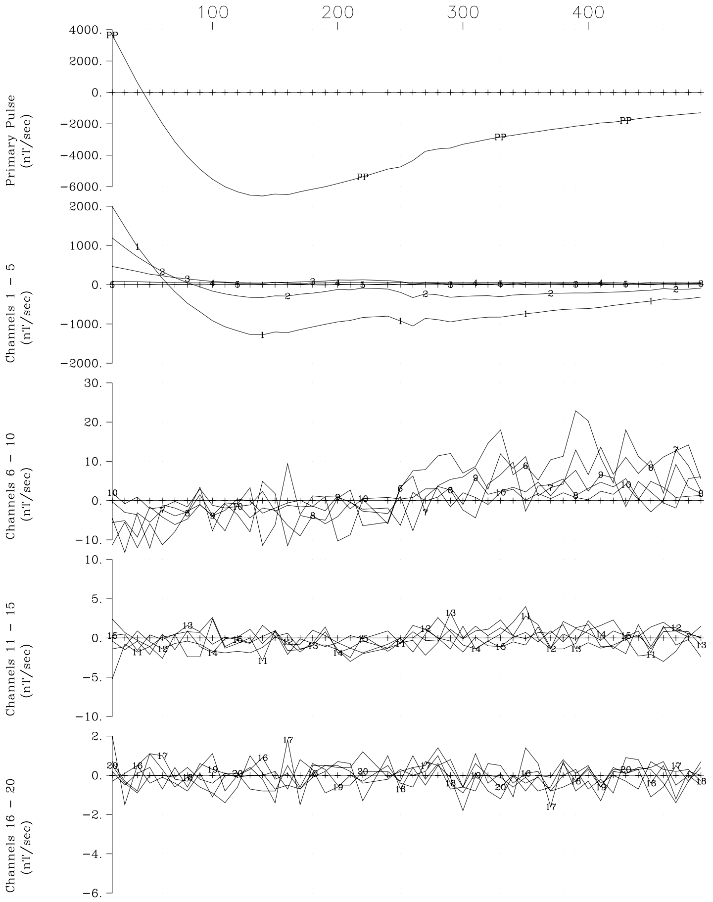
Transition Metals Sunday Lake Loop 2014-North, Hole SL-13-004 X Component Crone Geophysics & Exploration Ltd.
