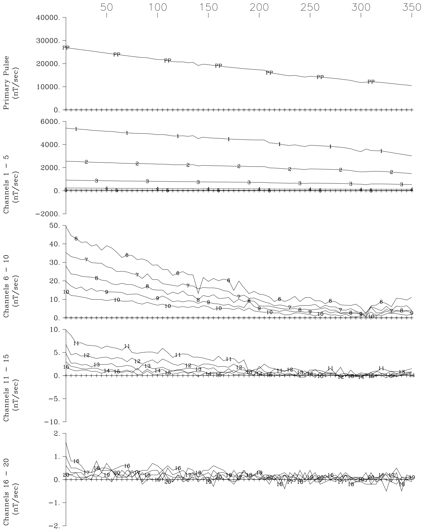
Transition Metals Sunday Lake Loop 2014-North, Hole SL-13-003 Z Component Crone Geophysics & Exploration Ltd.
