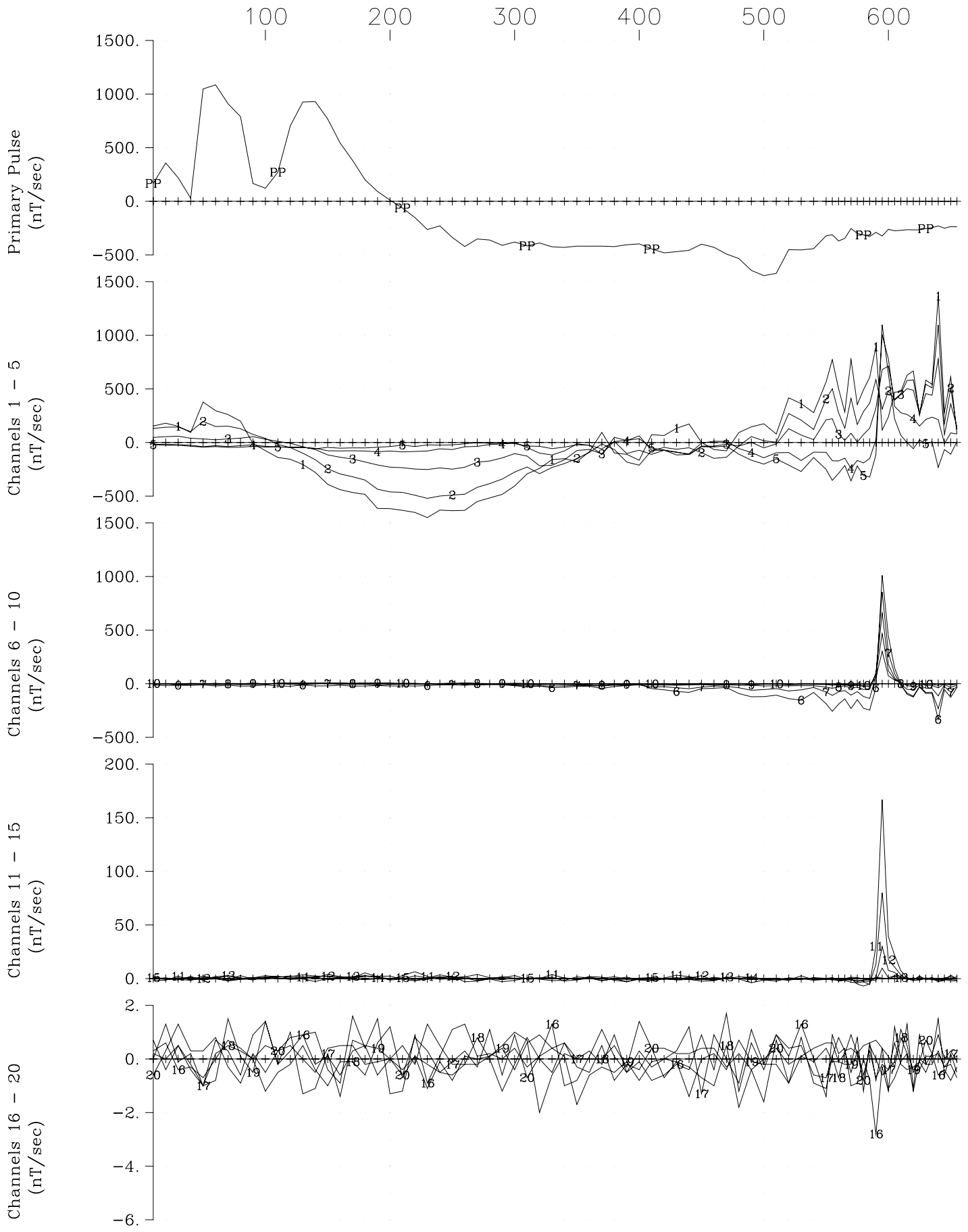
Transition Metals Sunday Lake Loop 2014-East, Hole SL-13-006 Y Component Crone Geophysics & Exploration Ltd.
