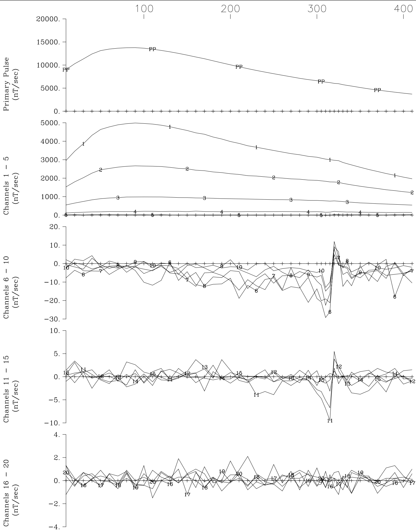
Transition Metals Sunday Lake Loop 2014-North, Hole SL-14-001 X Component Crone Geophysics & Exploration Ltd.
