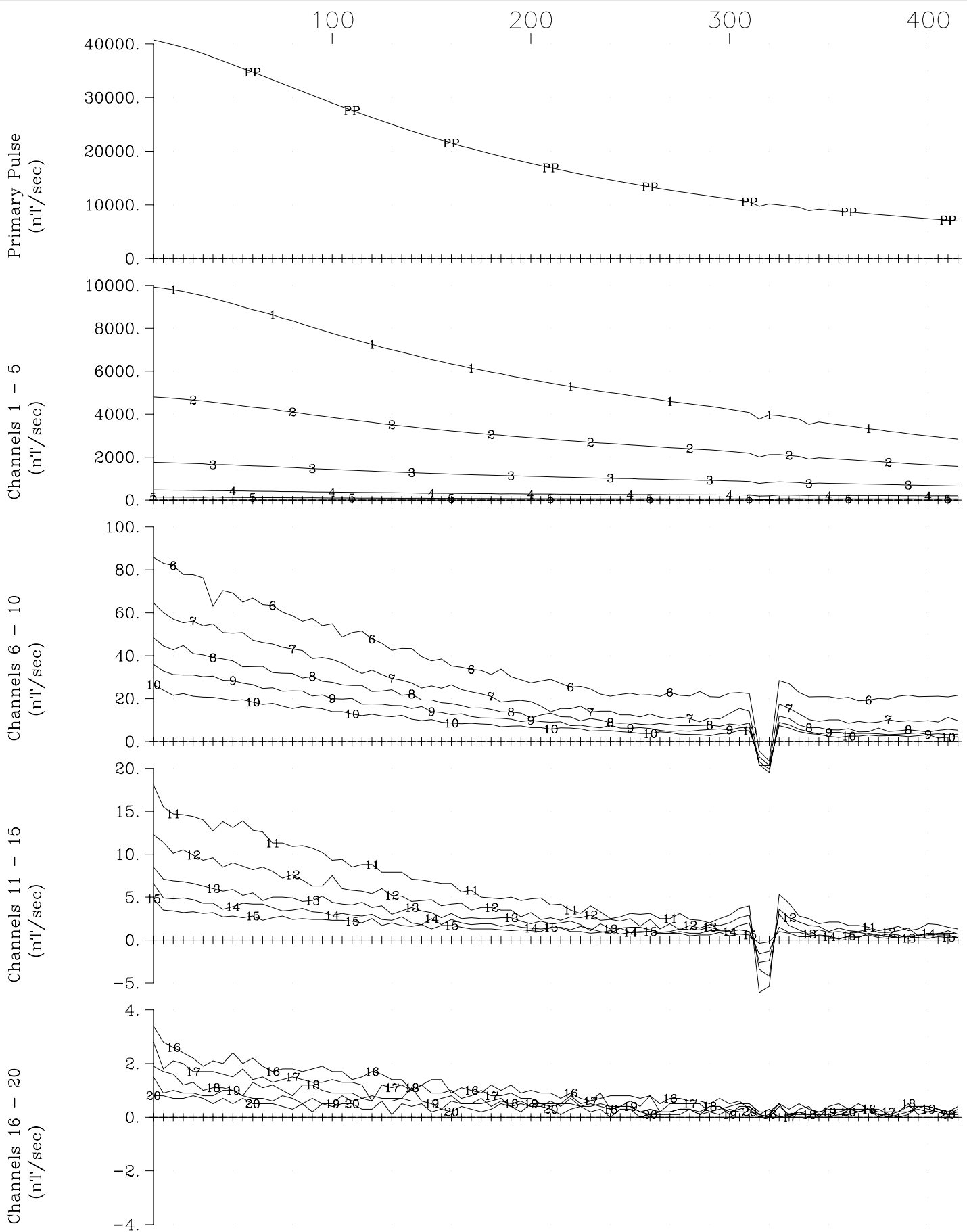
Transition Metals Sunday Lake Loop 2014-North, Hole SL-14-001 Z Component Crone Geophysics & Exploration Ltd.
