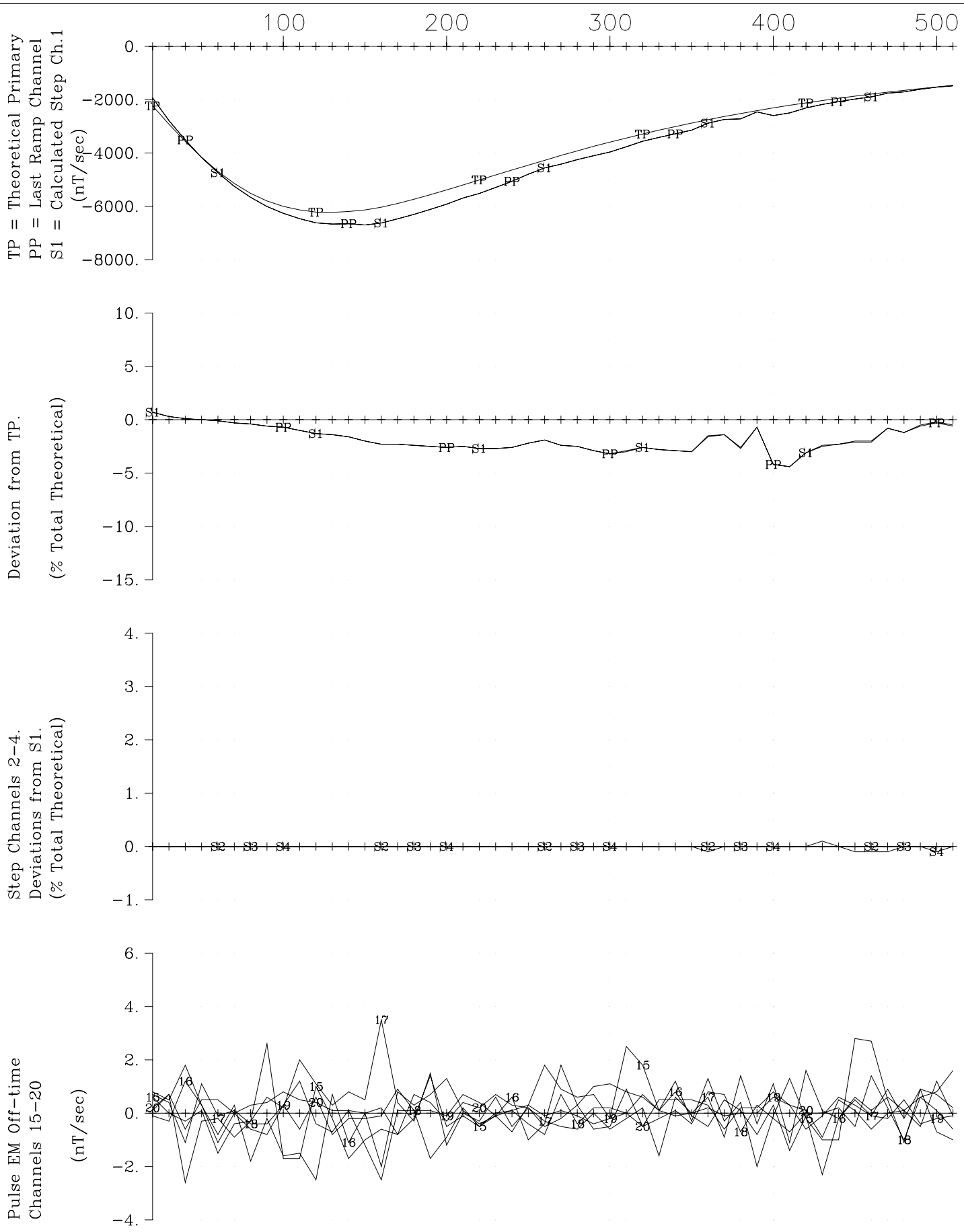
Transition Metals Sunday Lake Loop 2014-North, Hole SL-13-002 Y Component Crone Geophysics & Exploration Ltd.
