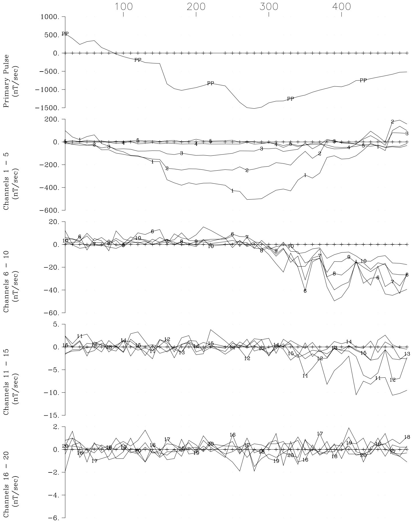
Transition Metals Sunday Lake Loop 2014-North, Hole SL-13-004 Y Component Crone Geophysics & Exploration Ltd.
