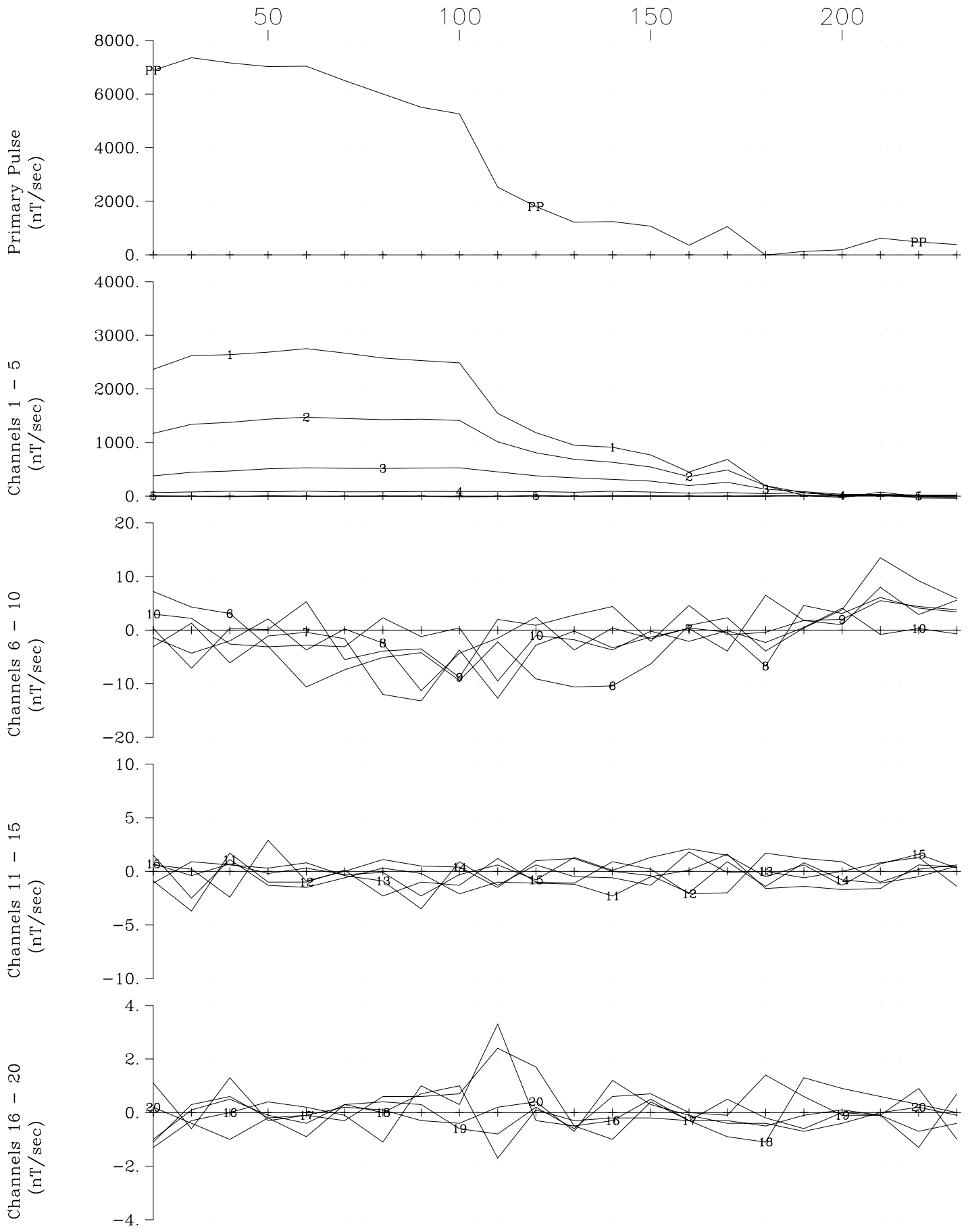
Transition Metals Sunday Lake Loop 2014-North, Hole SL-13-005 X Component Crone Geophysics & Exploration Ltd.
