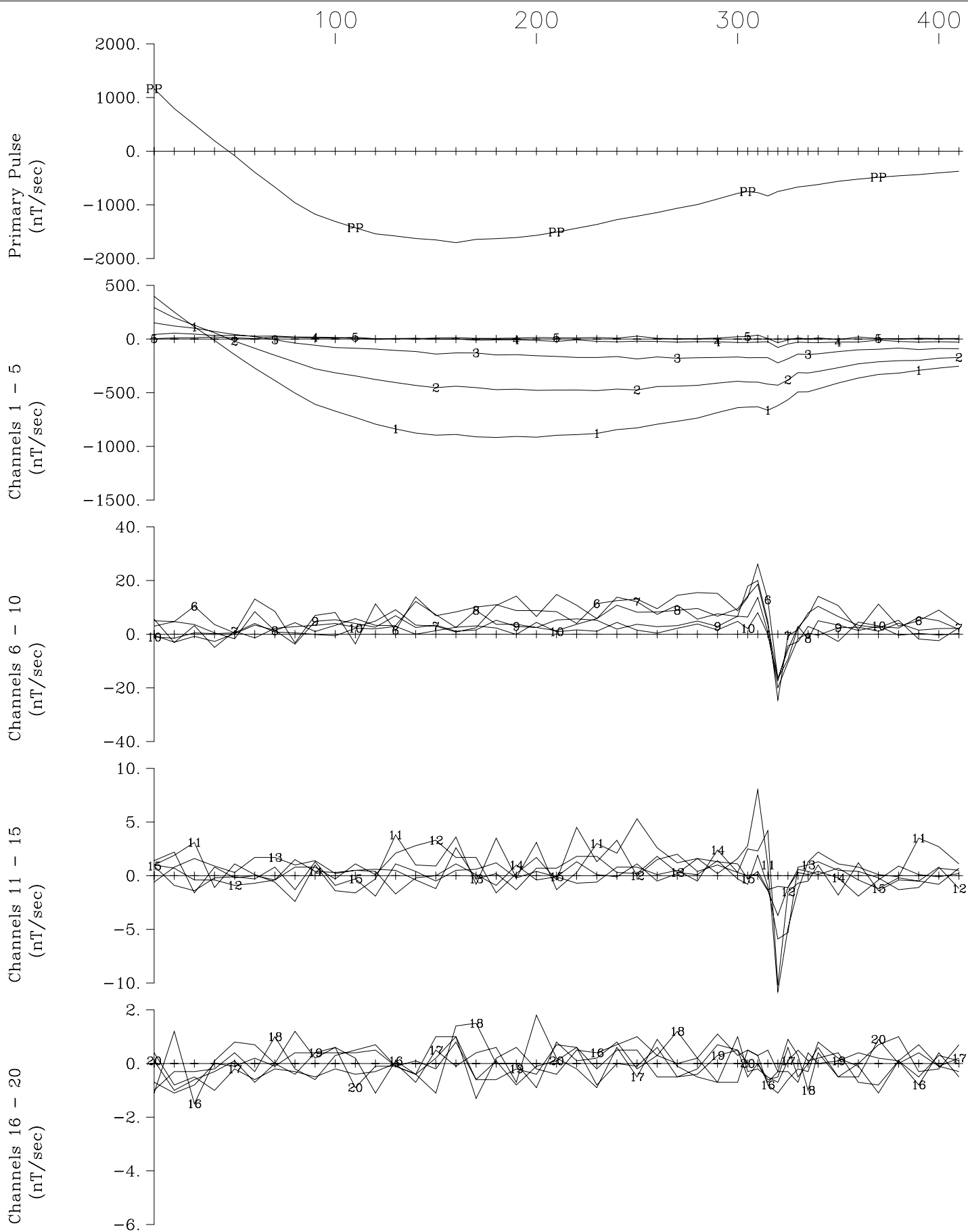
Transition Metals Sunday Lake Loop 2014-North, Hole SL-14-001 Y Component Crone Geophysics & Exploration Ltd.
