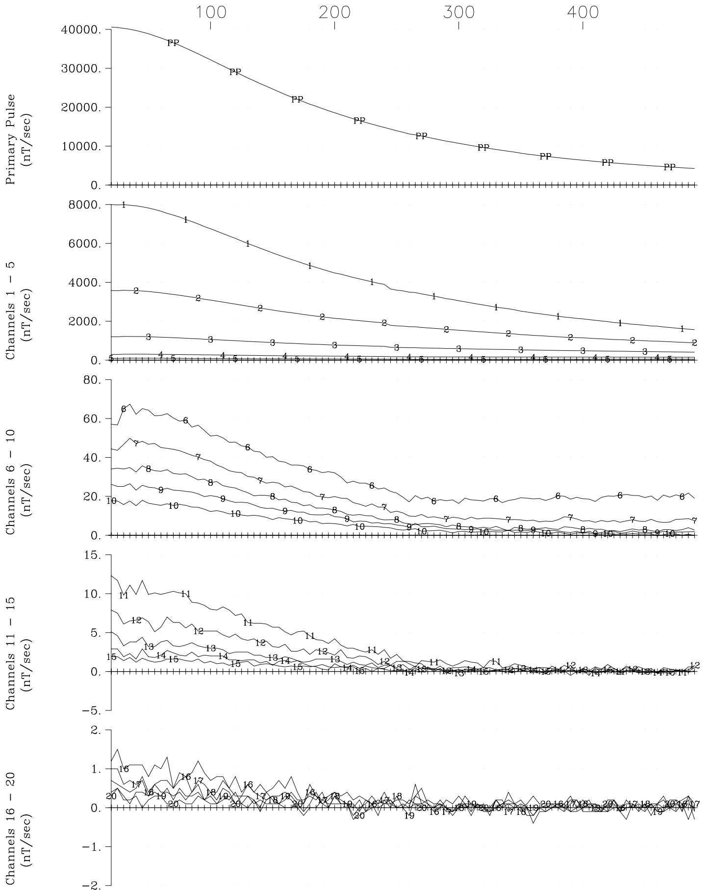
Transition Metals Sunday Lake Loop 2014-North, Hole SL-13-004 Z Component Crone Geophysics & Exploration Ltd.
