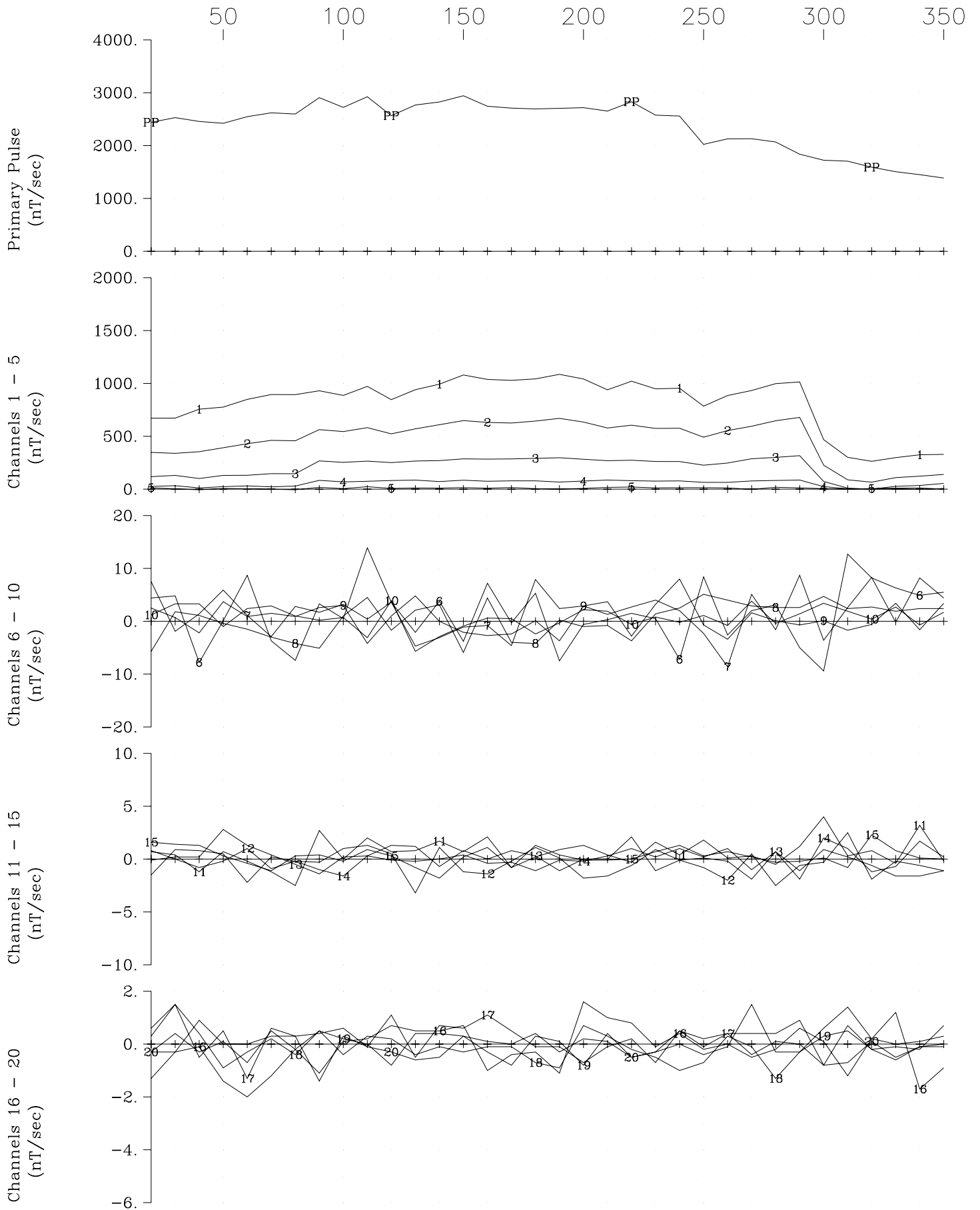
Transition Metals Sunday Lake Loop 2014-North, Hole SL-13-003 Y Component Crone Geophysics & Exploration Ltd.
