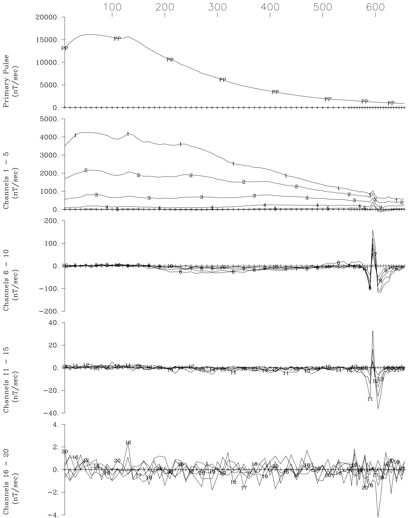
Transition Metals Sunday Lake Loop 2014-East, Hole SL-13-006 X Component Crone Geophysics & Exploration Ltd.
