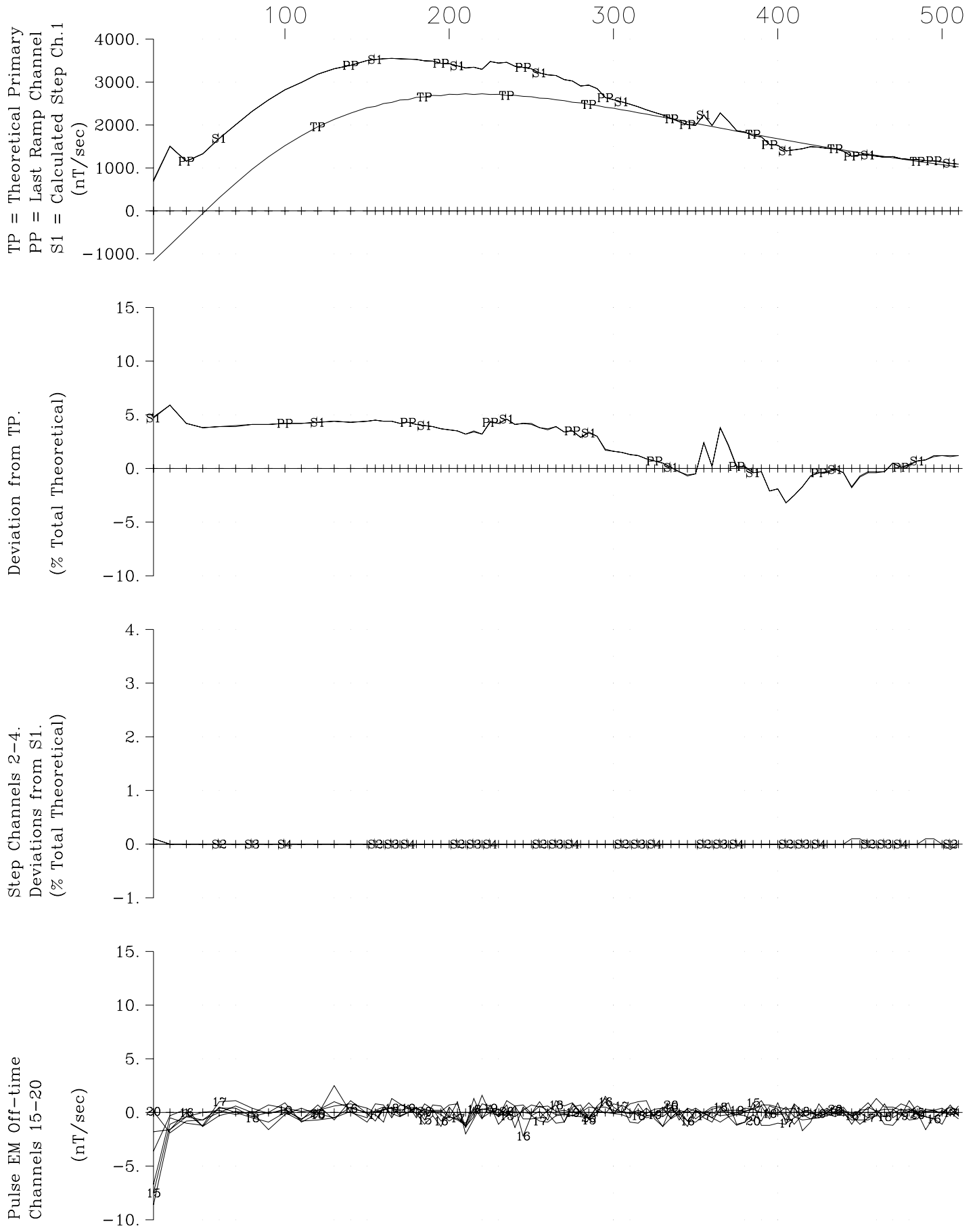
Transition Metals Sunday Lake Loop 2014-East, Hole SL-13-002 Y Component Crone Geophysics & Exploration Ltd.
