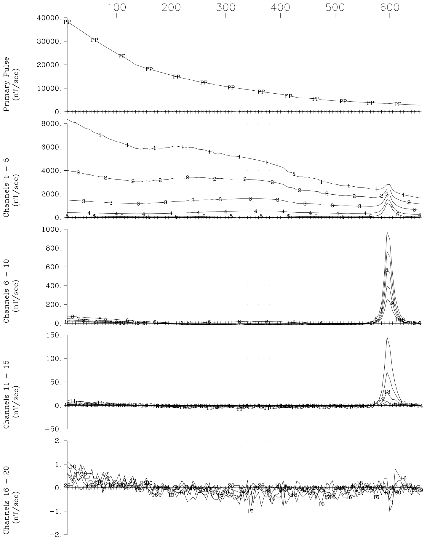
Transition Metals Sunday Lake Loop 2014-East, Hole SL-13-006 Z Component Crone Geophysics & Exploration Ltd.
