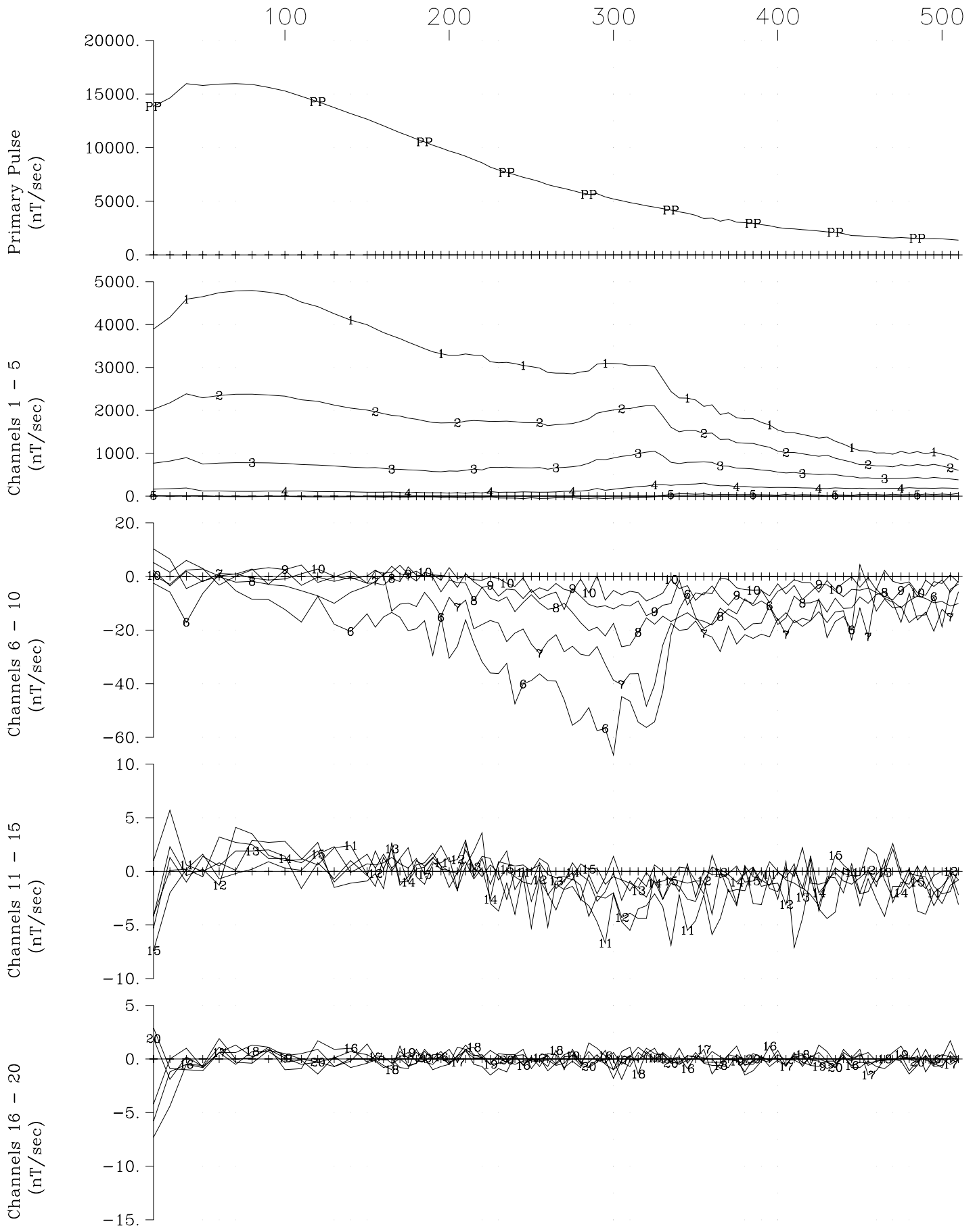
Transition Metals Sunday Lake Loop 2014-East, Hole SL-13-002 X Component Crone Geophysics & Exploration Ltd.
