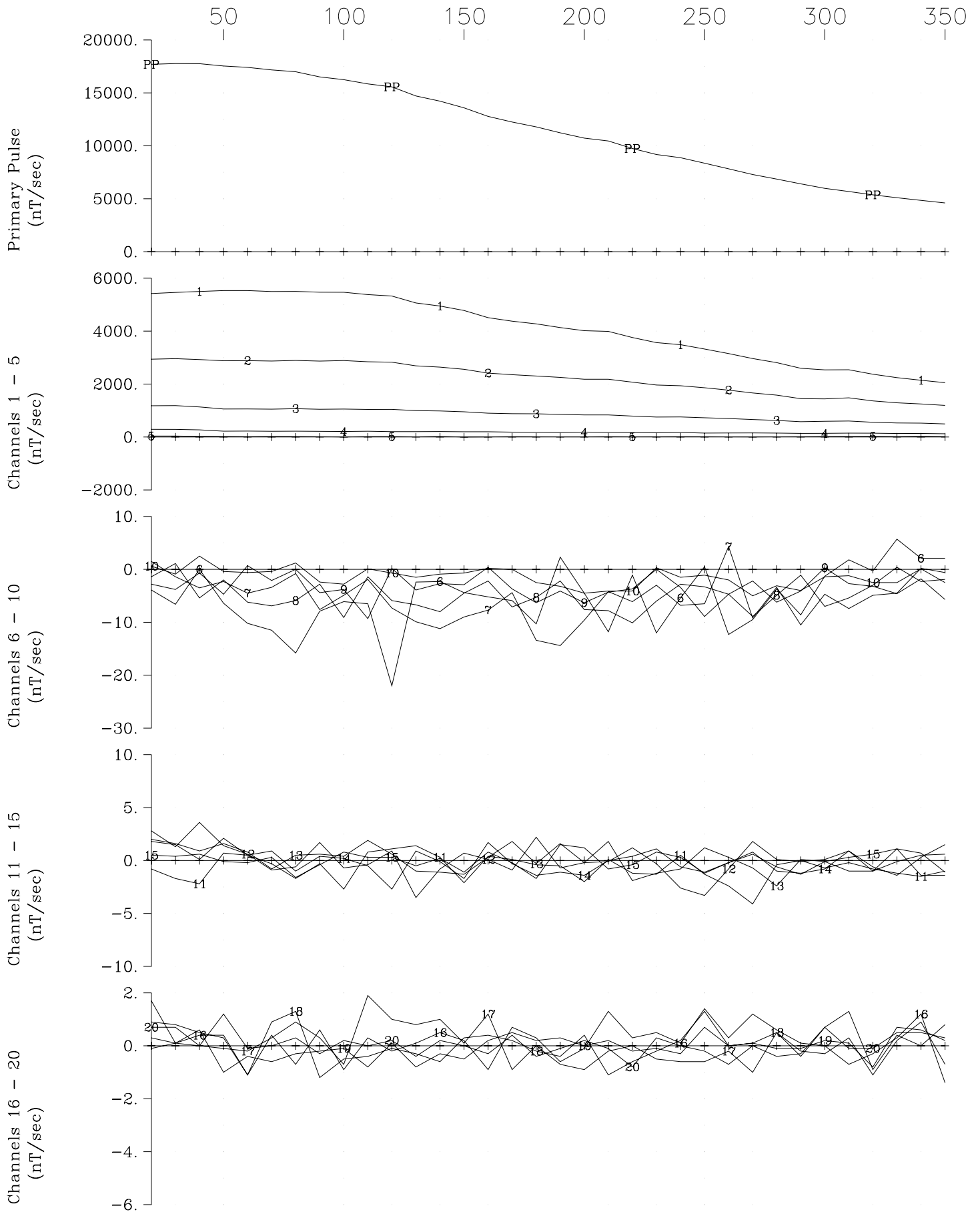
Transition Metals Sunday Lake Loop 2014-North, Hole SL-13-003 X Component Crone Geophysics & Exploration Ltd.
