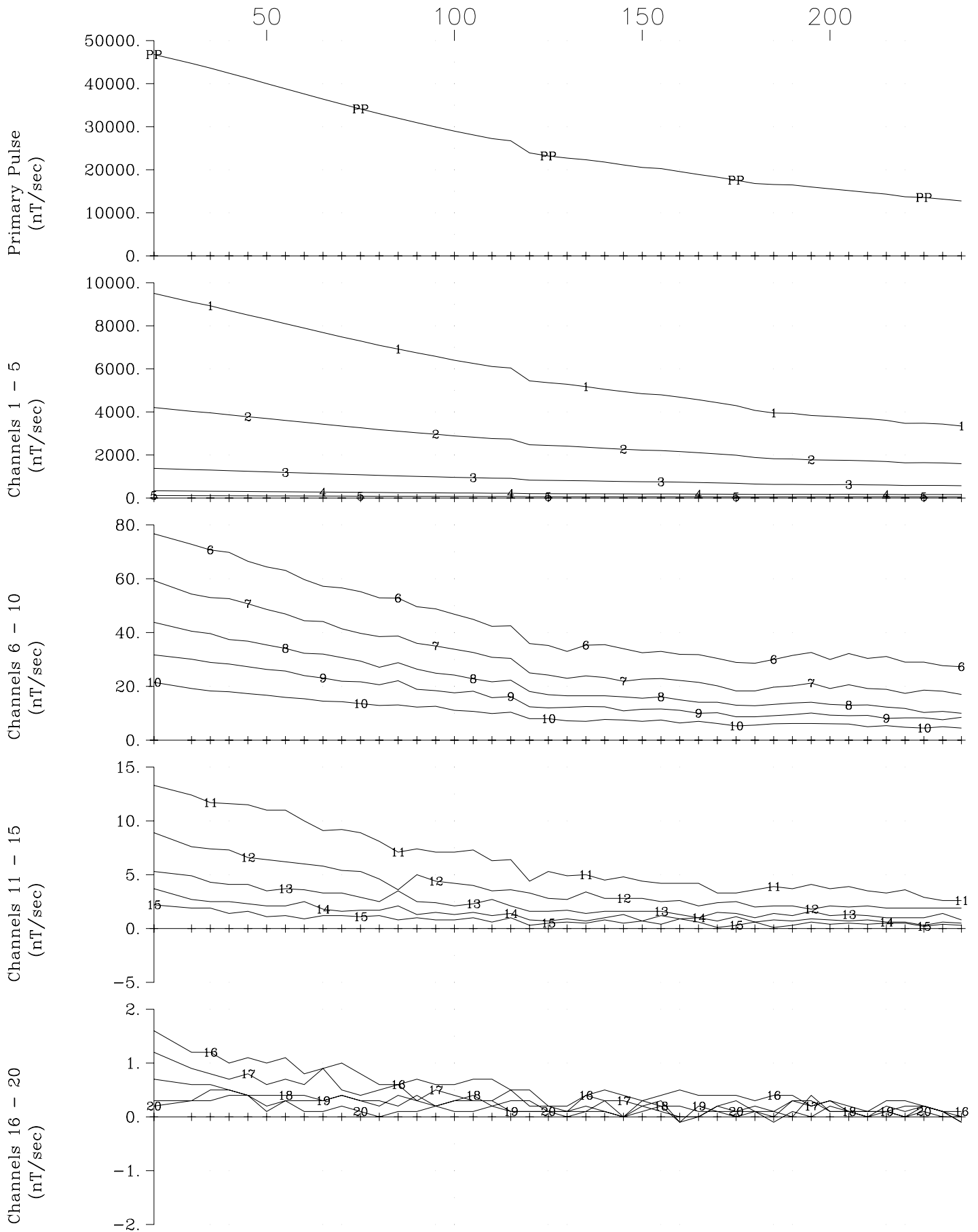
Transition Metals Sunday Lake Loop 2014-North, Hole SL-13-005 Z Component Crone Geophysics & Exploration Ltd.
