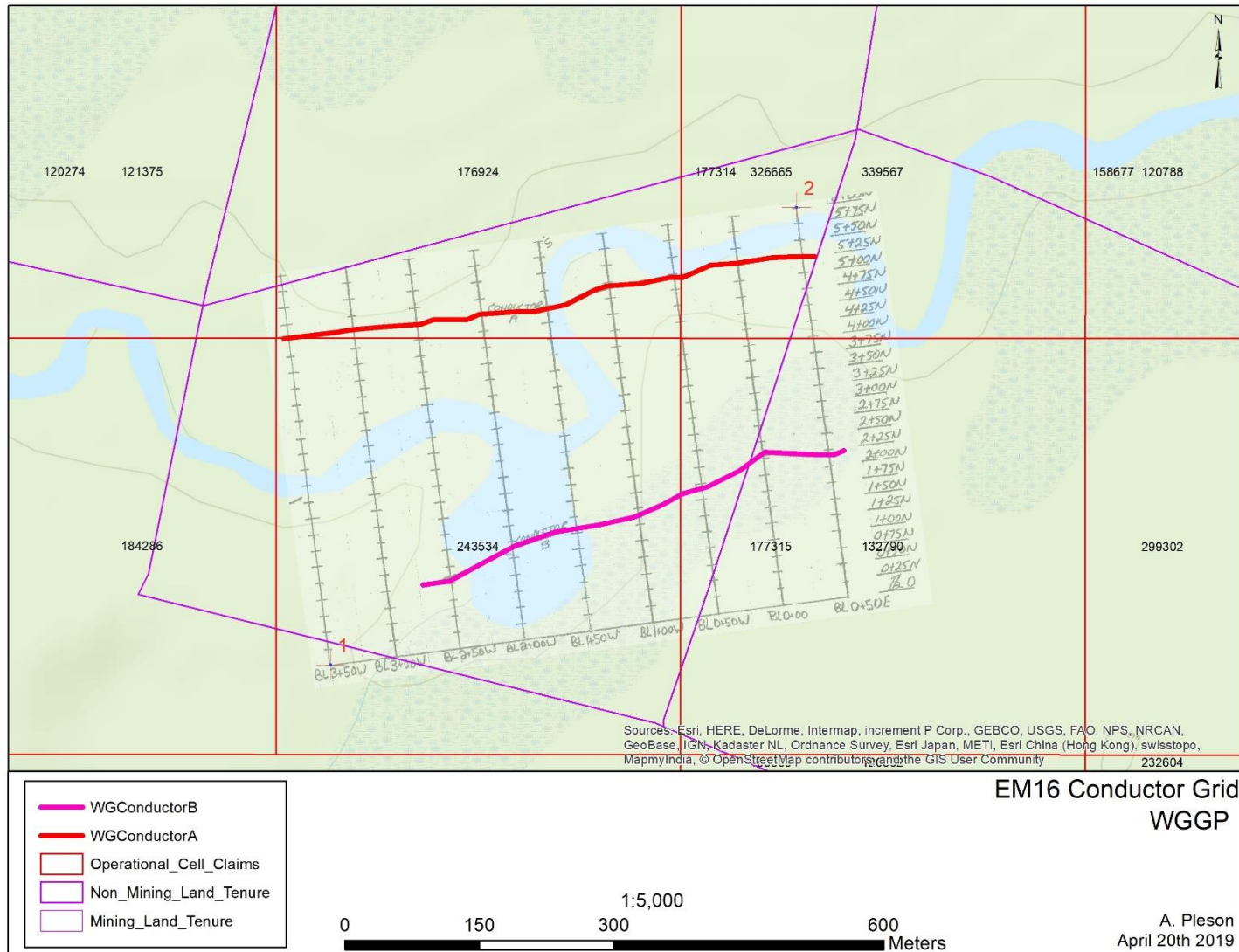
Figure 5: VLF Final Map
