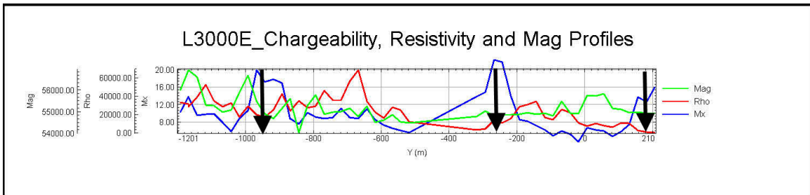
Figure 4.16a: L3000E Chargeability, Resistivity and Mag Profiles
