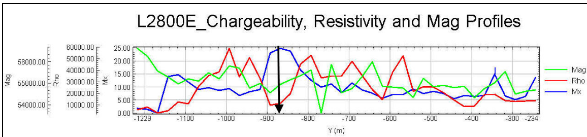
Figure 4.14a: L2800E Chargeability, Resistivity and Mag Profiles
