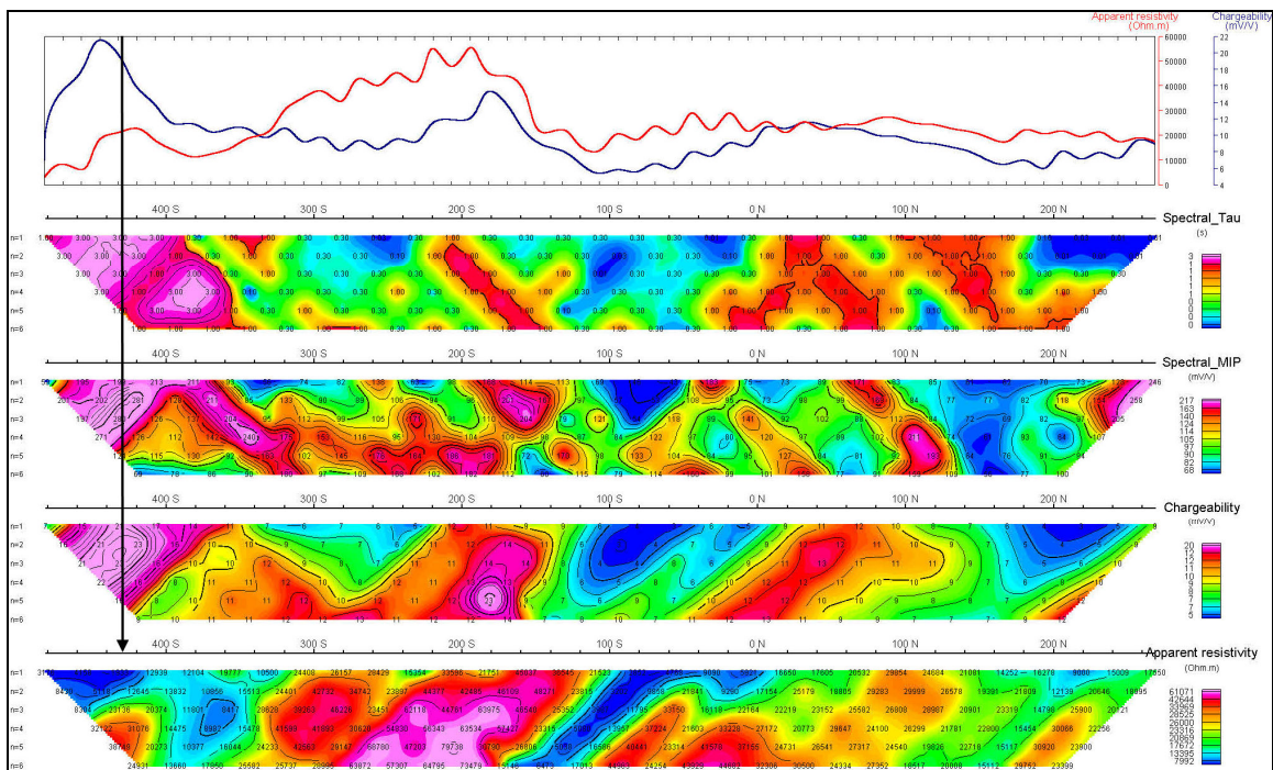
Figure 4.10b: Zoomed in Anomaly from L2300E Pseudosection
