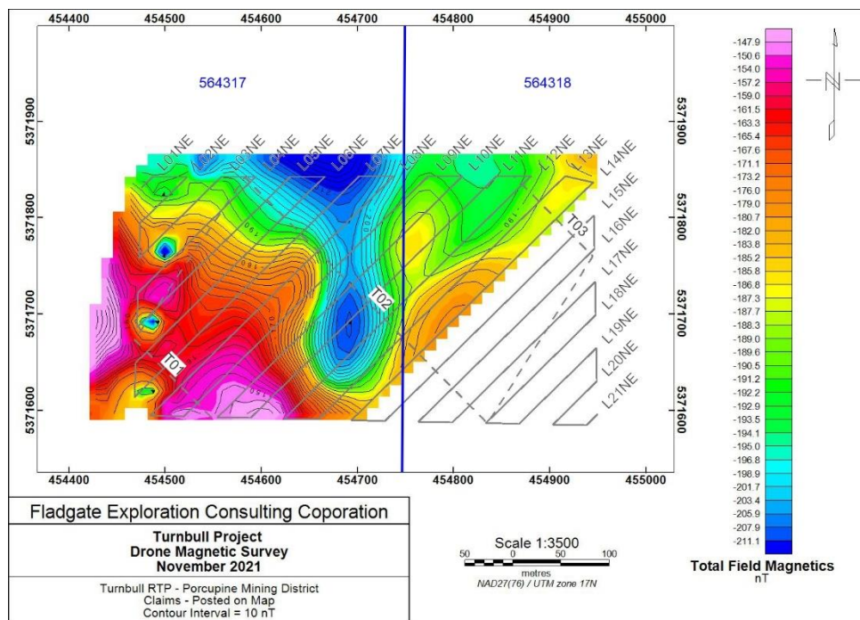
Figure 6 – Map of Total Field Magnetics
