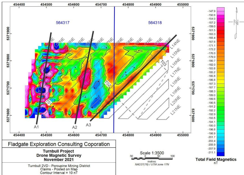
Figure 8 – 2 nd Vertical Derivative Map
