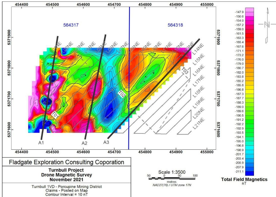
Figure 7 – 1 st Vertical Derivative Map
