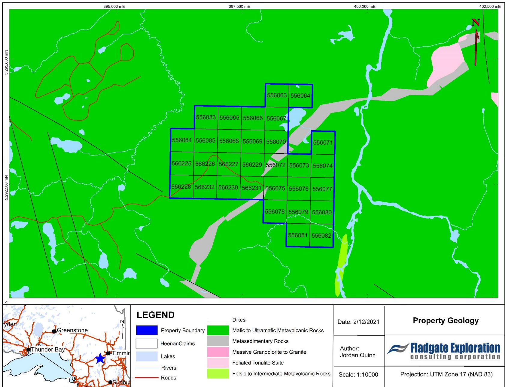
Figure 4 - Heenan Property Geology
