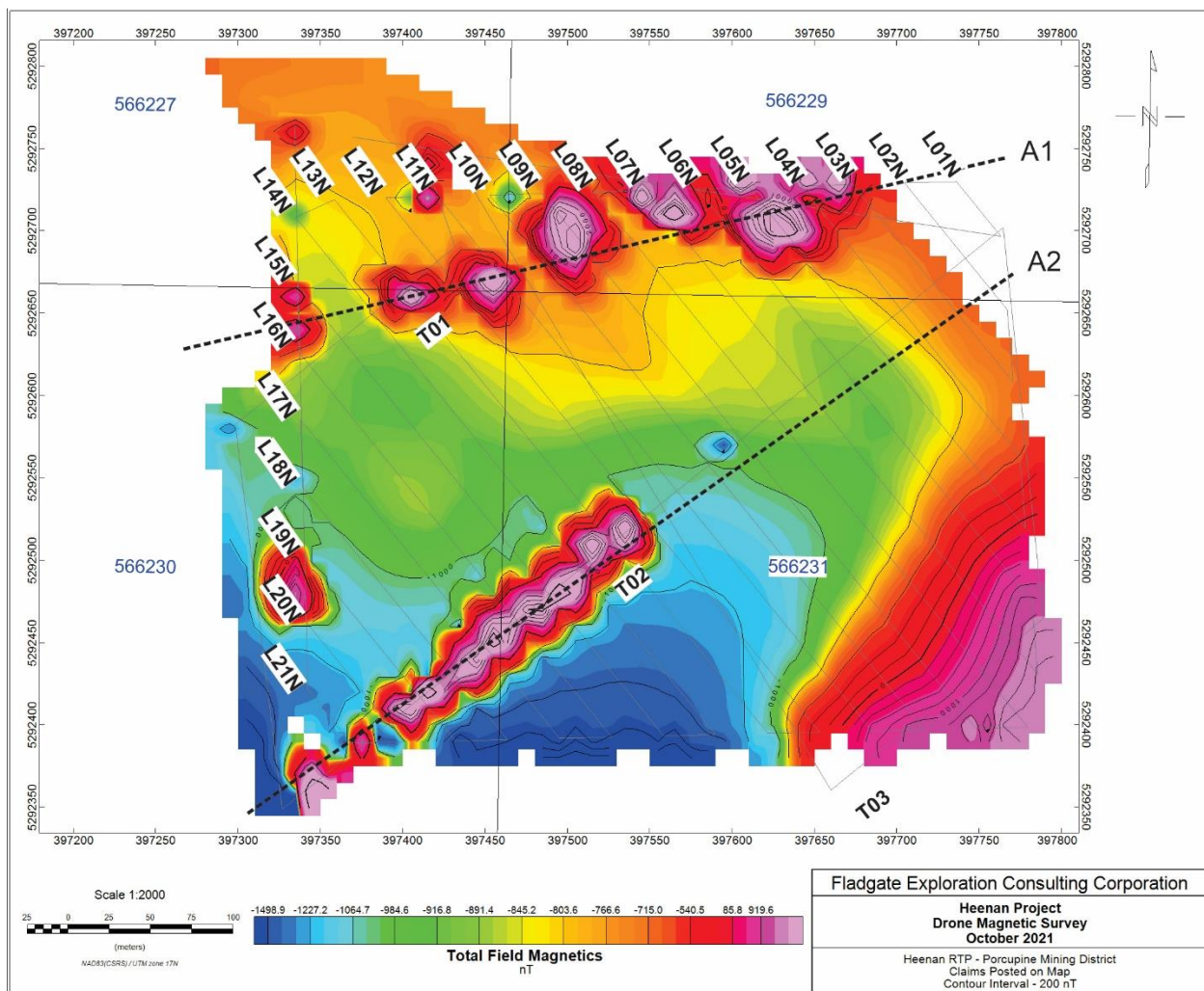
Figure 6 – Map of Total Field Magnetics
