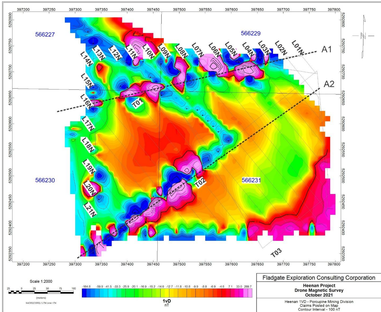
Figure 7 – 1 st Vertical Derivative Map
