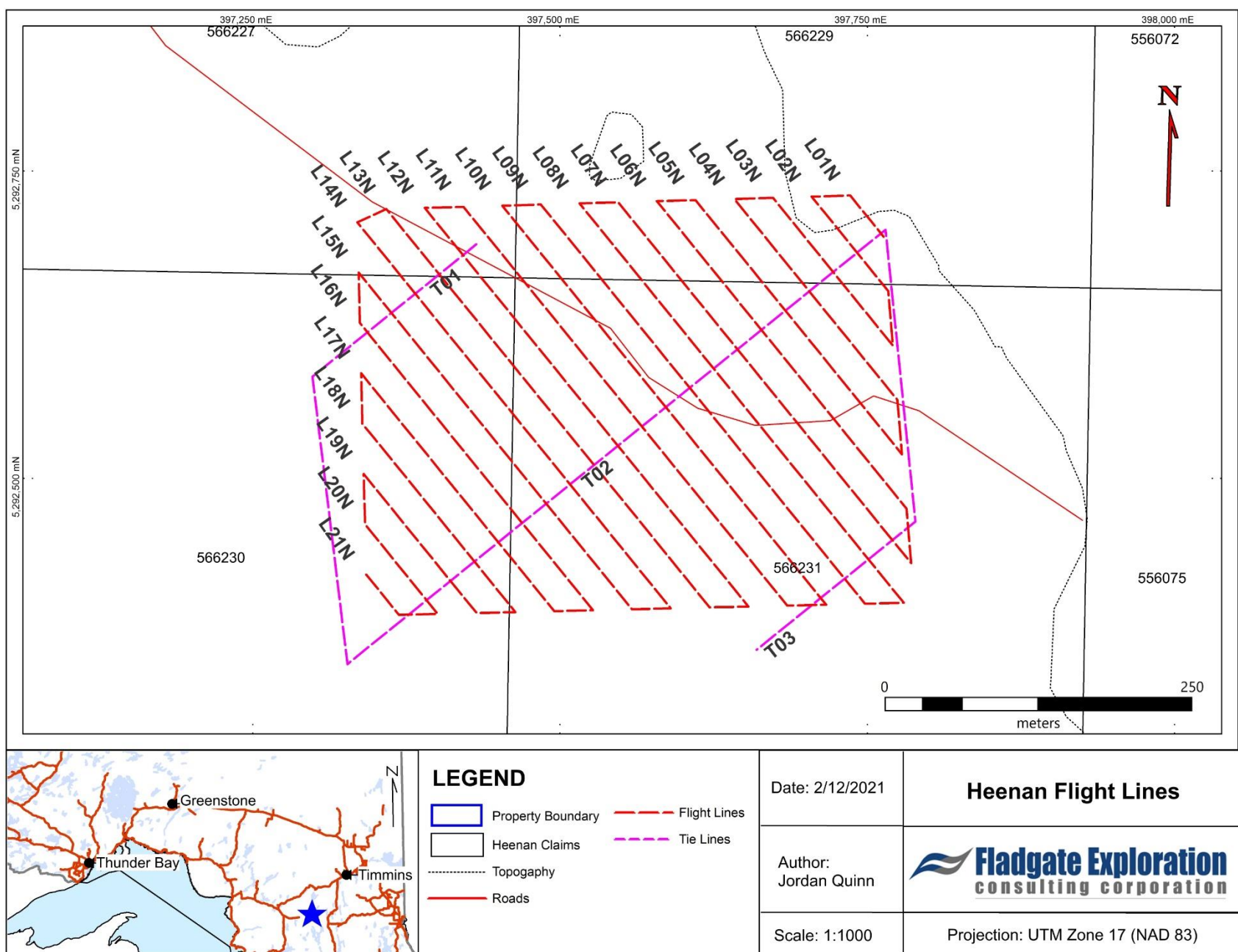
Figure 5 – Map of Heenan Drone Survey
