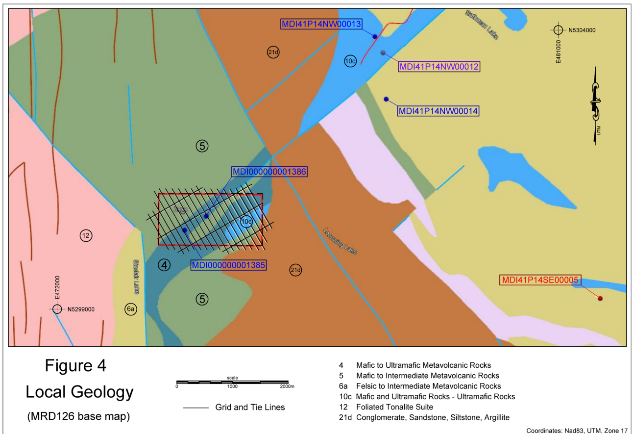
Figure 4 – Local Geology
