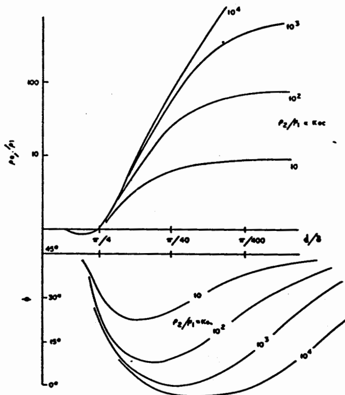
Figure 9. Variations of amplitude |\rho_a/\rho_1| and phase \phi for two-layer earth with resistive basement (after Cagniard (1953)).
