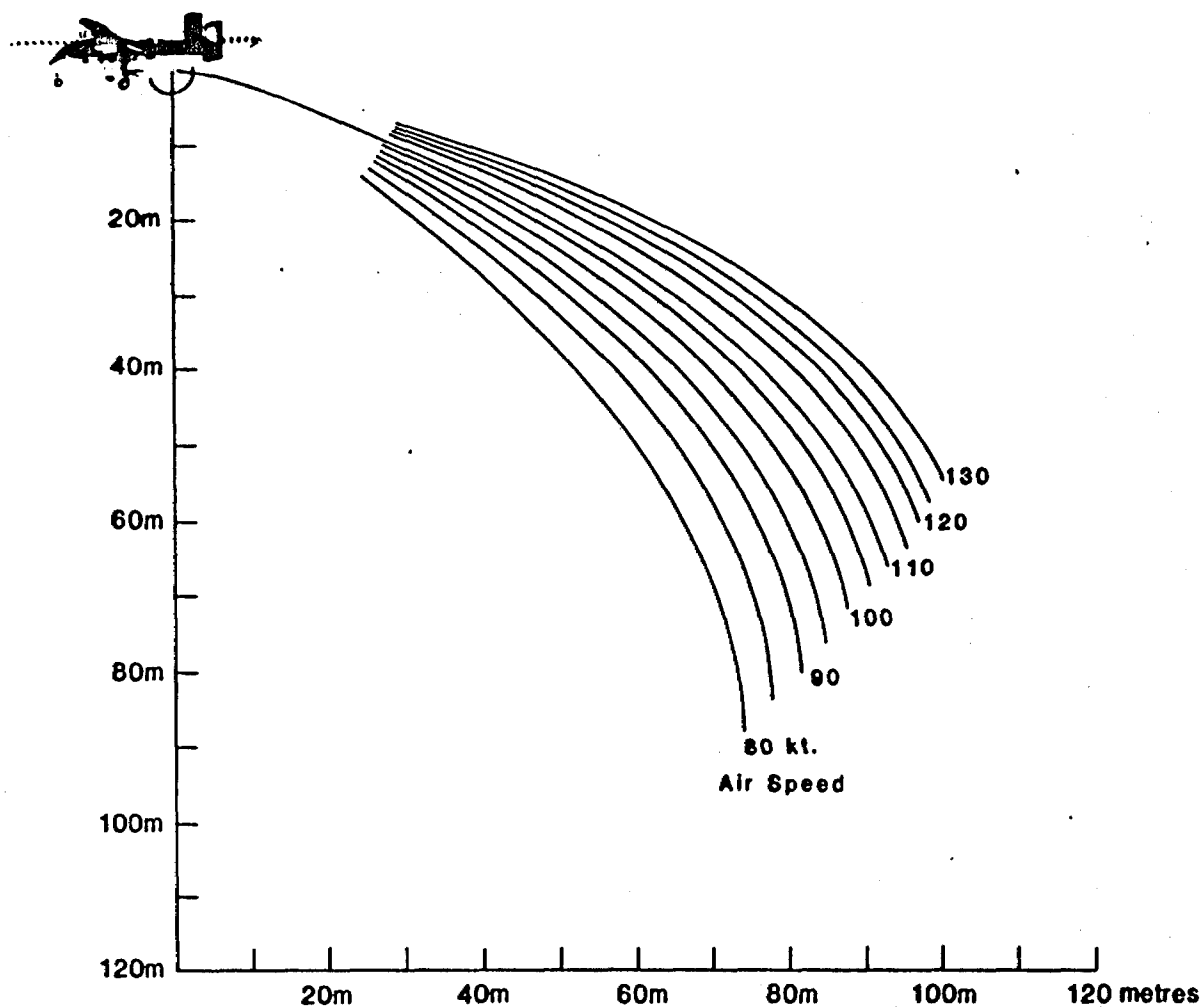
EFFECT OF AIR SPEED ON BIRD POSITION
