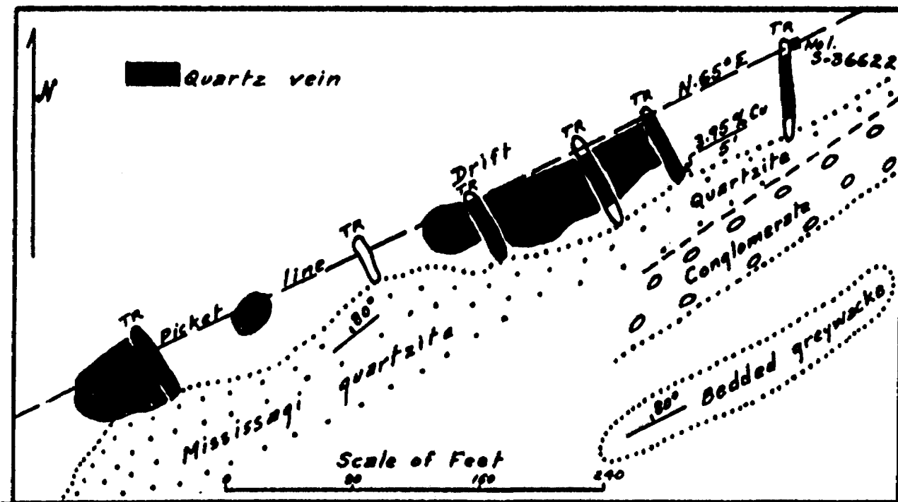
Geological sketch map of the quartz-chalcopyrite vein on claim S-36622, lot 7, con. 6, Baldwin township.
