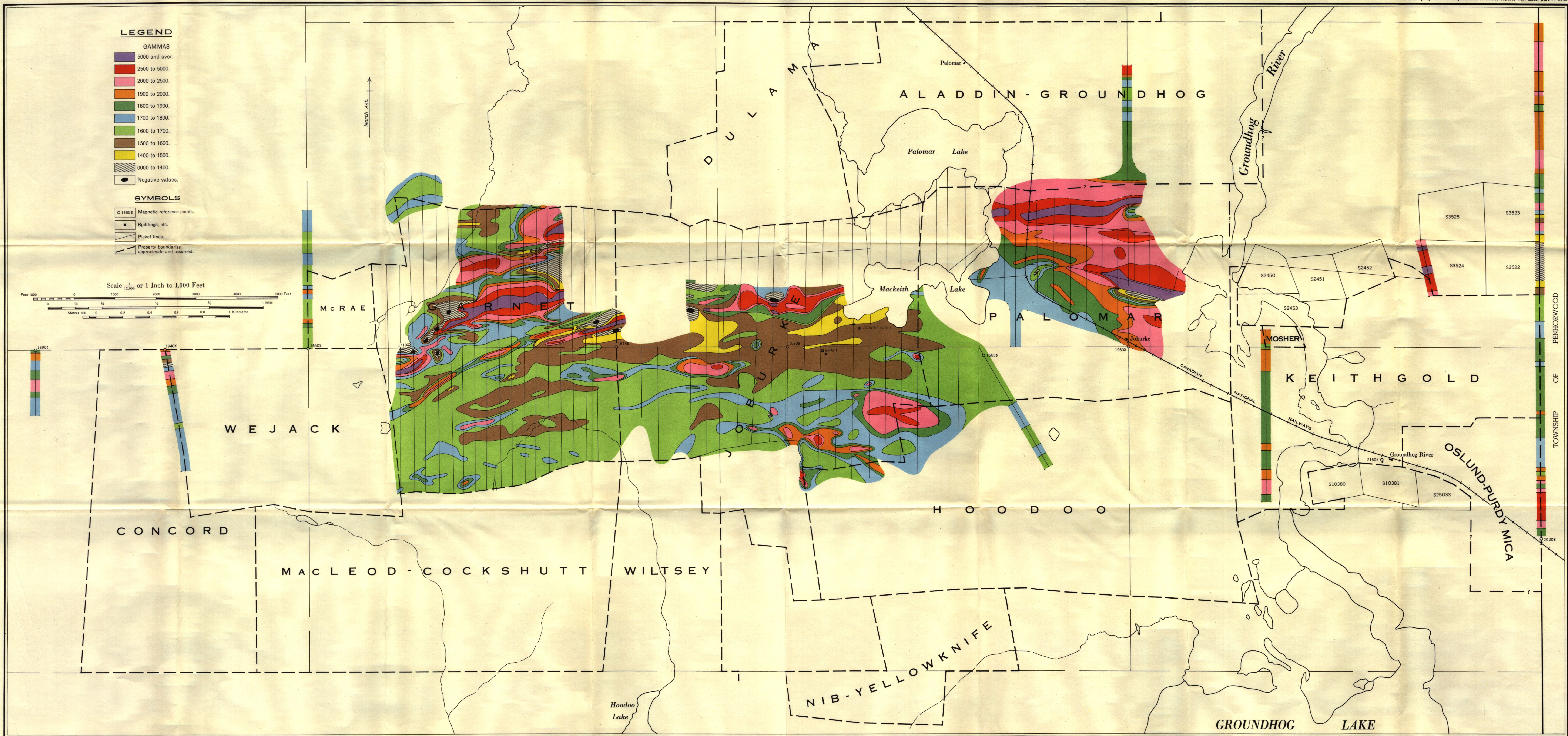
GROUND MAGNETIC CONTOUR MAP OF THE JOBURKE AREA, KEITH TOWNSHIP, DISTRICT OF SUDBURY, ONTARIO.
