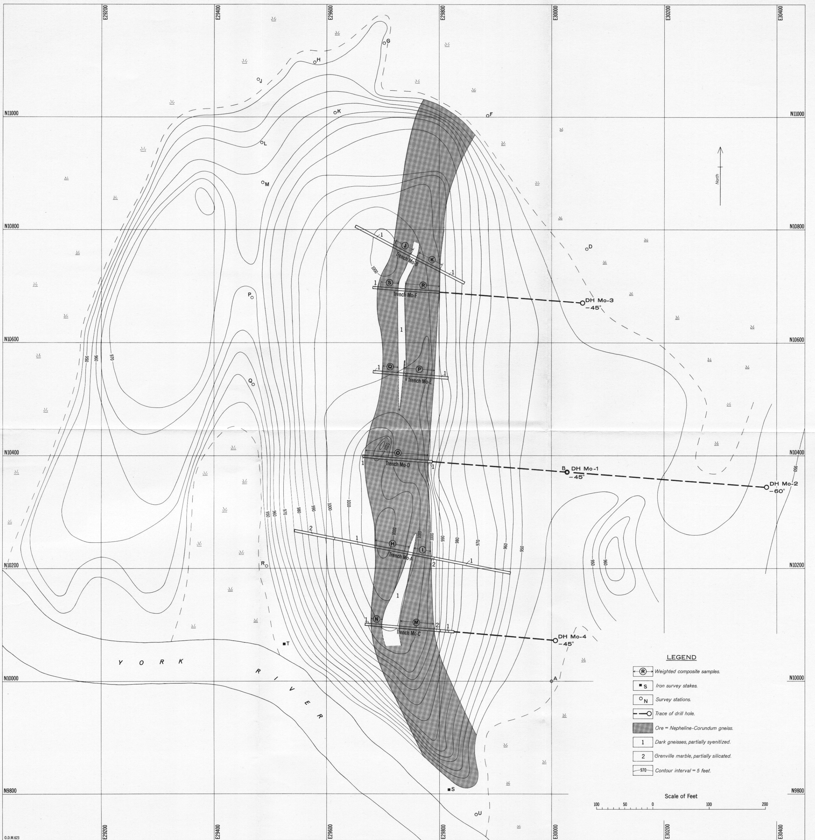
Surface plan showing the Nepheline and Corundum deposit, Monteagle Minerals Ltd. Monteagle Township, Ontario.
