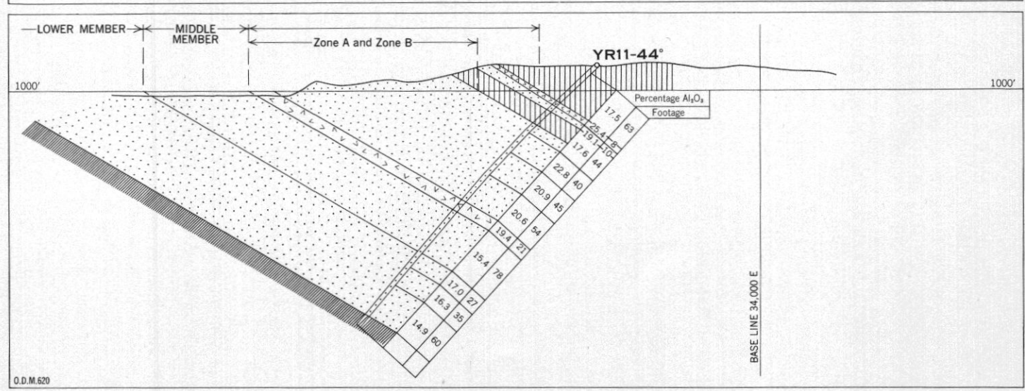
Drill sections through the York River nepheline band
