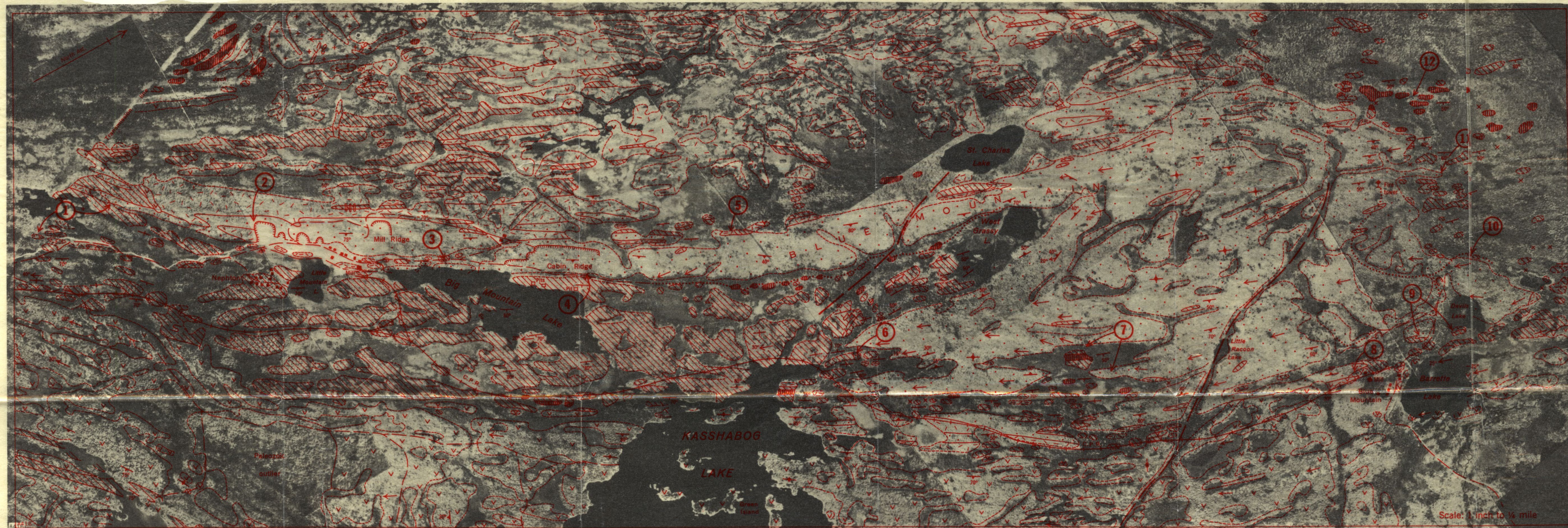
OVERPRINT SHOWING GEOLOGY OF THE BLUE MOUNTAIN NEPHELINE SYENITE AERIAL PHOTOGRAPH OF THE BLUE MOUNTAIN NEPHELINE SYENITE, METHUEN TOWNSHIP, PETERBOROUGH COUNTY
