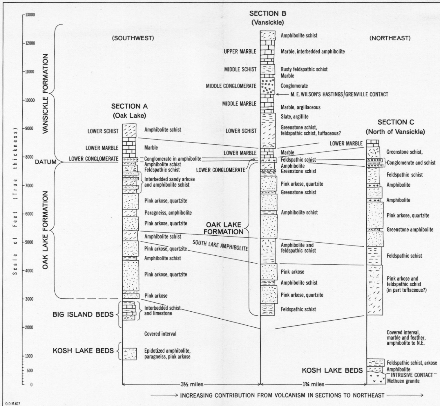
Sections of the sedimentary formations, southeastern Methuen Township
