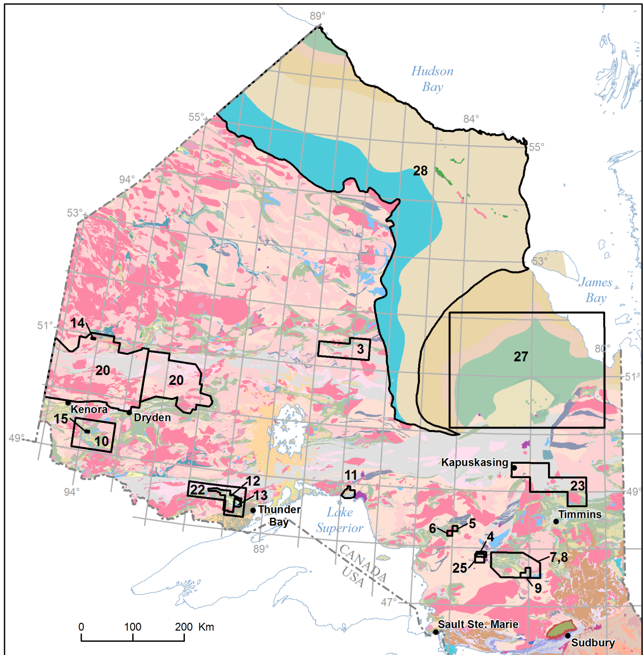
Location of the Earth Resources and Geoscience Mapping Section projects in northern Ontario and the Far North of Ontario as described in Summary of Field Work and Other Activities, 2016 . Numbers correspond to article numbers.
