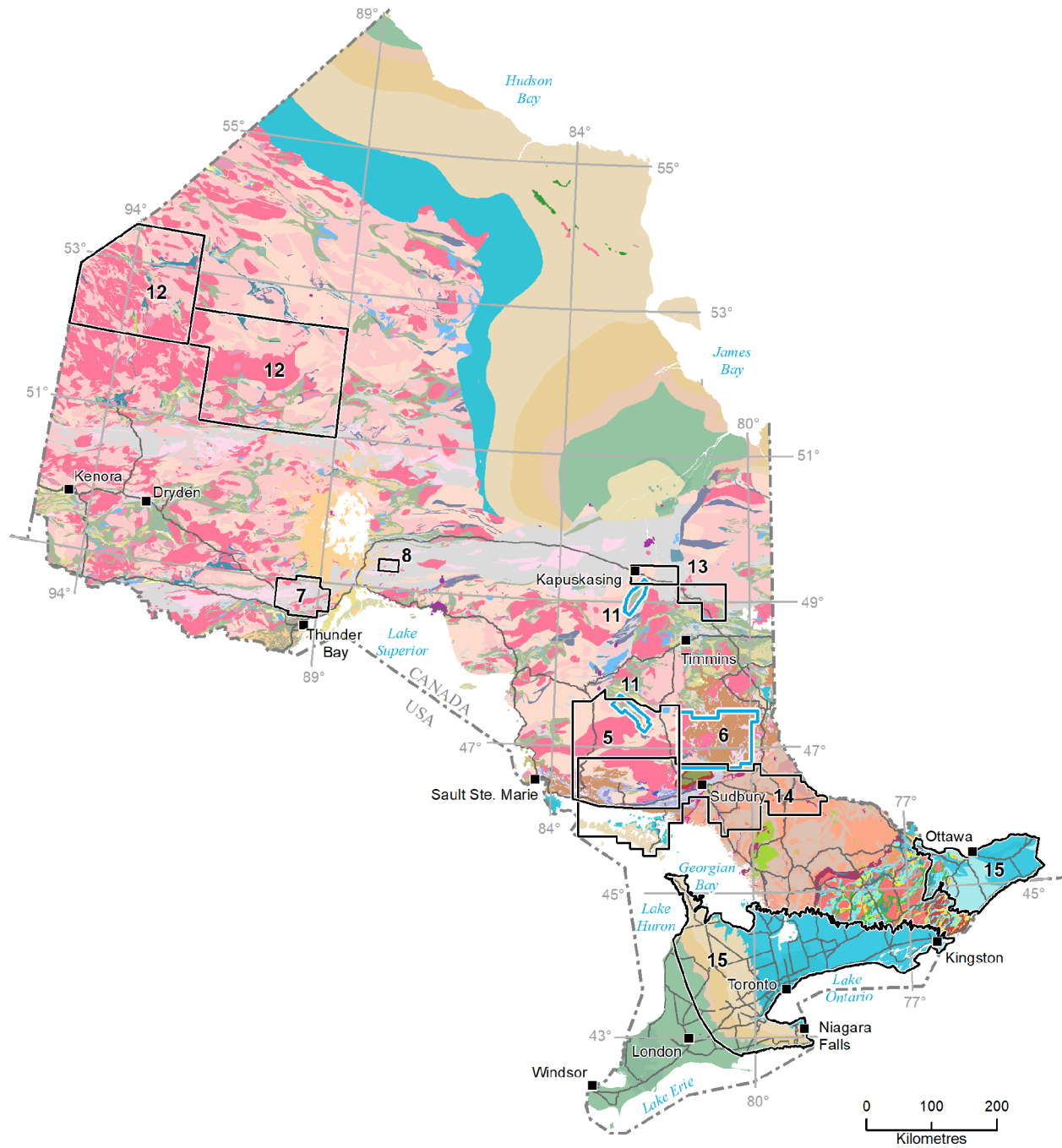
Locations of the Ontario Geological Survey projects in Ontario as described in Summary of Field Work and Other Activities, 2020 . Numbers correspond to article numbers; note articles 1 to 4, 9, 10 and 16 are provincial in scope and are not indicated on the figure. Bedrock geology from Ontario Geological Survey (2011: Miscellaneous Release—Data 126—Revision 1).
