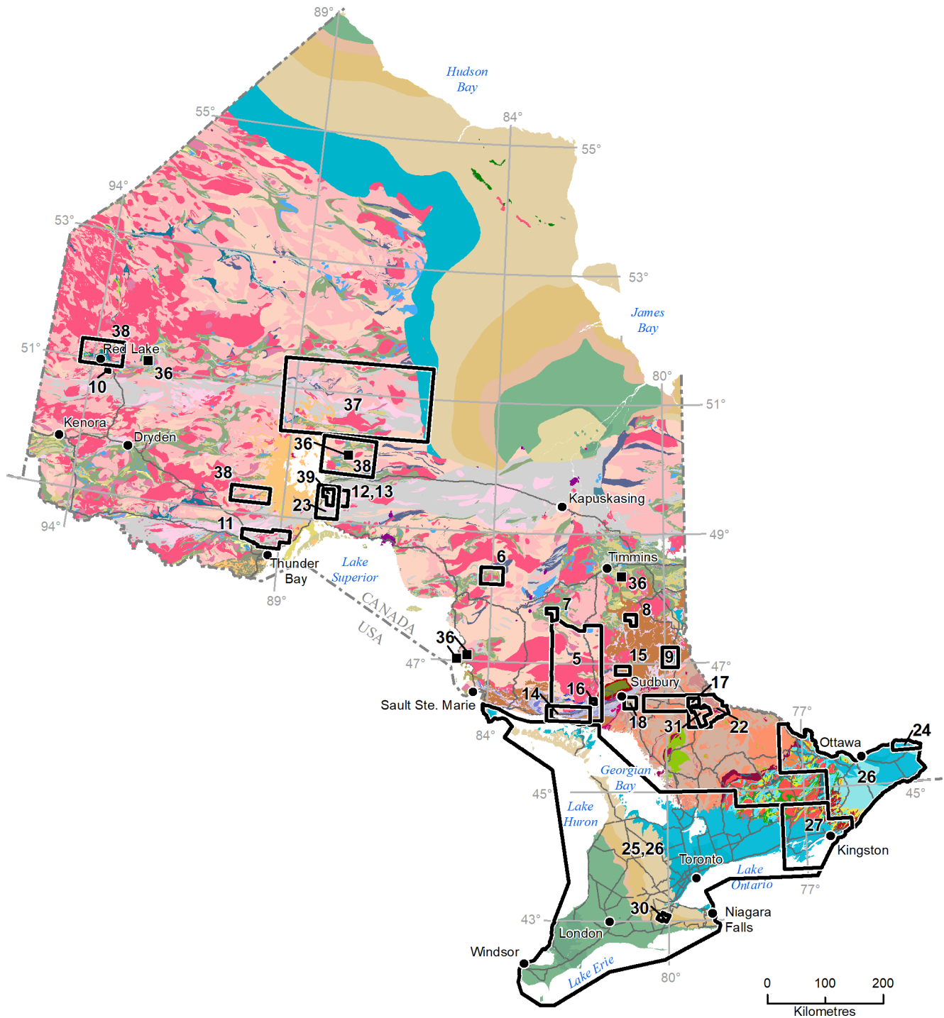
Locations of the Ontario Geological Survey projects in Ontario as described in Summary of Field Work and Other Activities, 2023 . Numbers correspond to article numbers; note, articles 1 to 4, 19, 20, 21, 28, 29, and 32 to 35 are provincial in scope and are not indicated on the figure. Bedrock geology from Ontario Geological Survey (2011: Miscellaneous Release—Data 126 – Revision 1).
