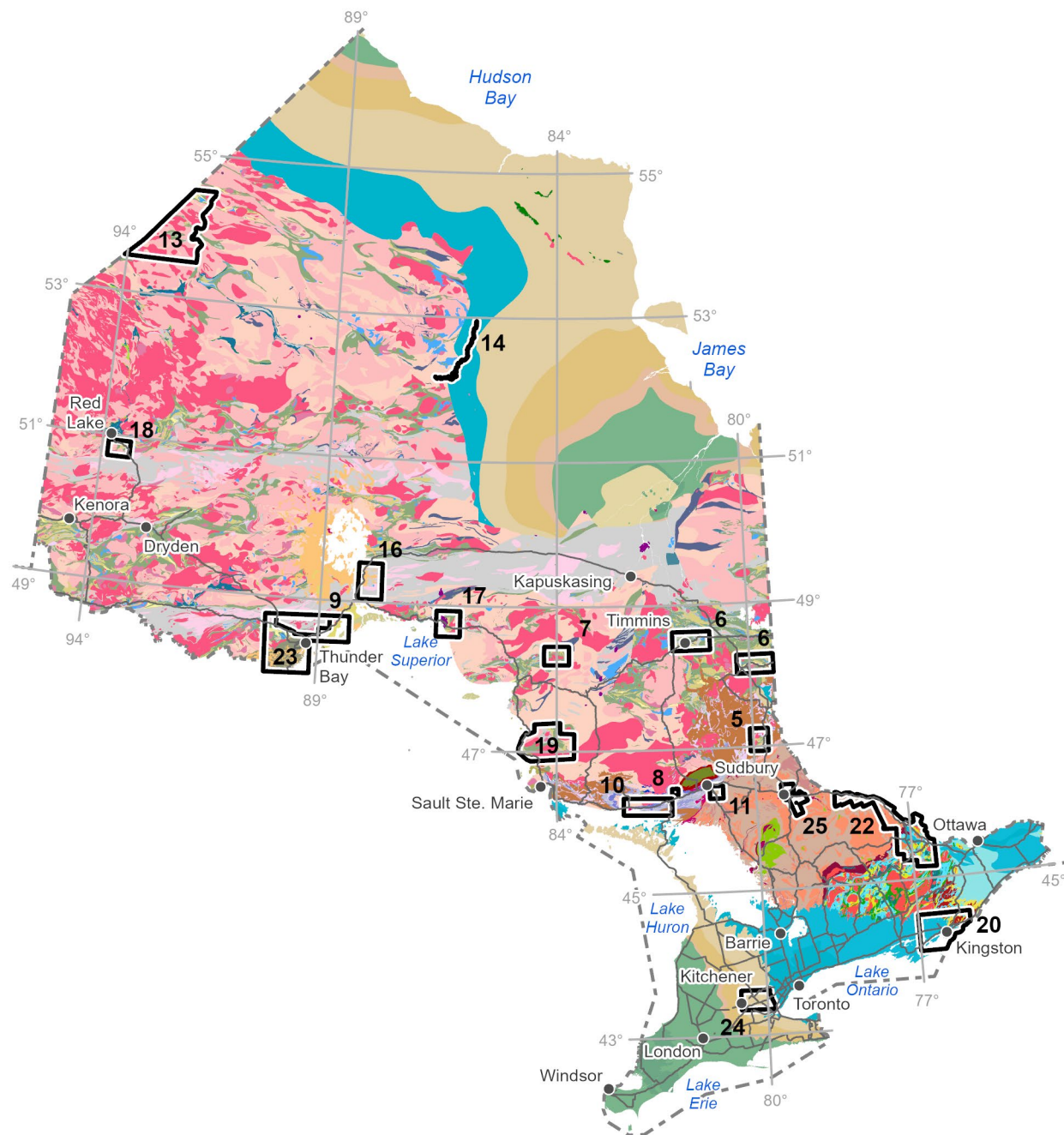
Locations of the Ontario Geological Survey projects in Ontario as described in Summary of Field Work and Other Activities, 2024 . Numbers correspond to article numbers; note, articles 1 to 4, 12, 15, 21, and 26 to 30 are provincial in scope and are not indicated on the figure. Bedrock geology from Ontario Geological Survey (2011: Miscellaneous Release—Data 126 – Revision 1).
